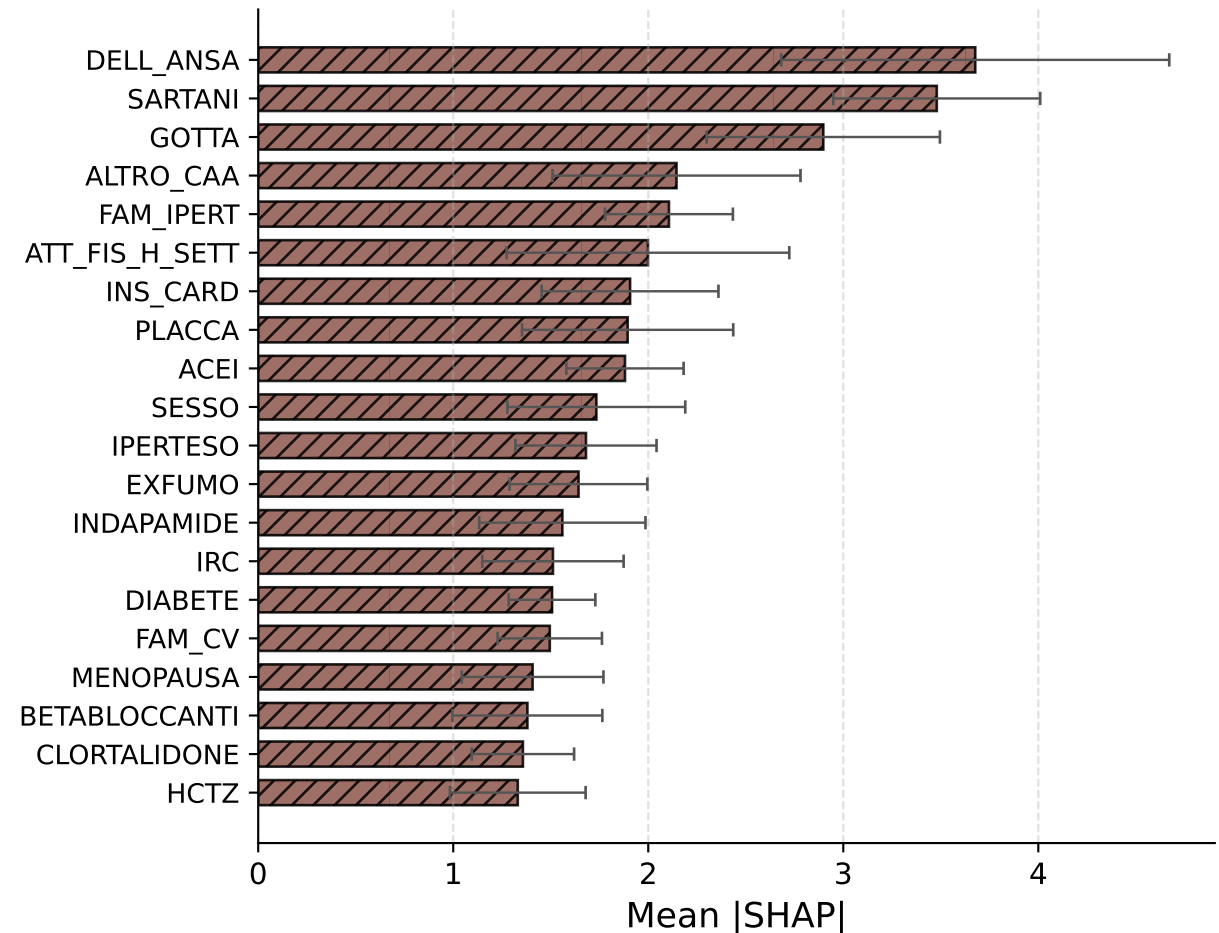
TabICL - RSF
