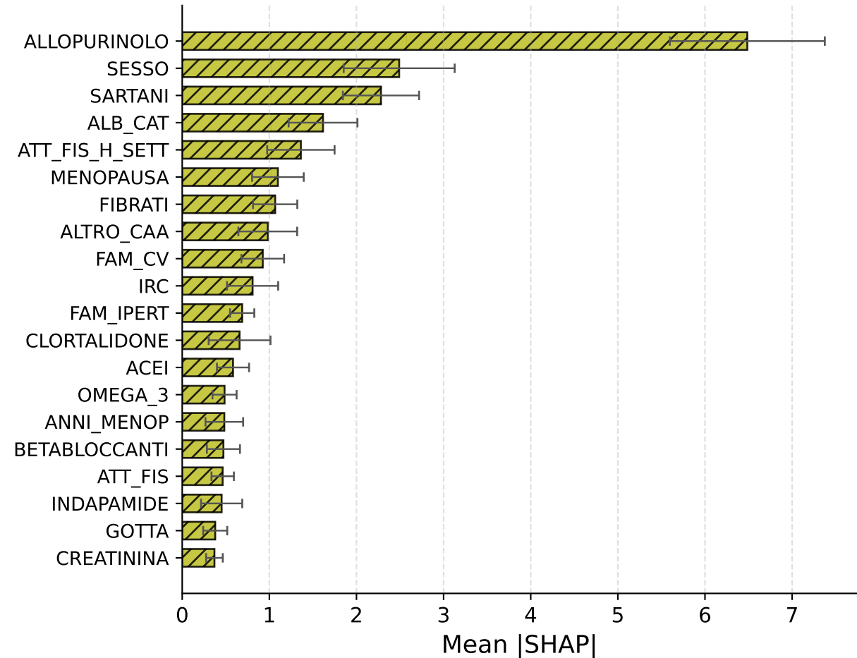
TabICL - Cox
