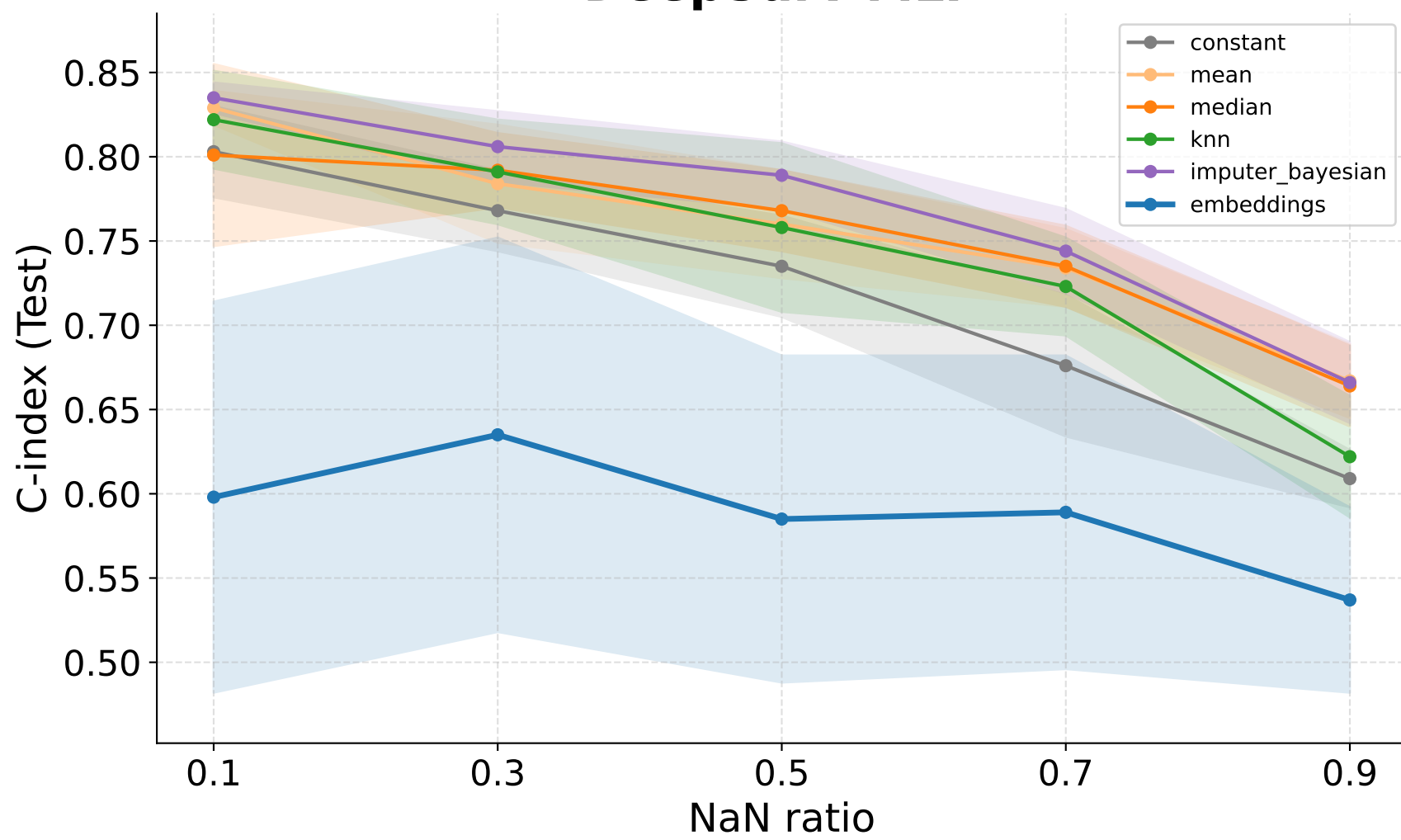
DeepSurv MLP
