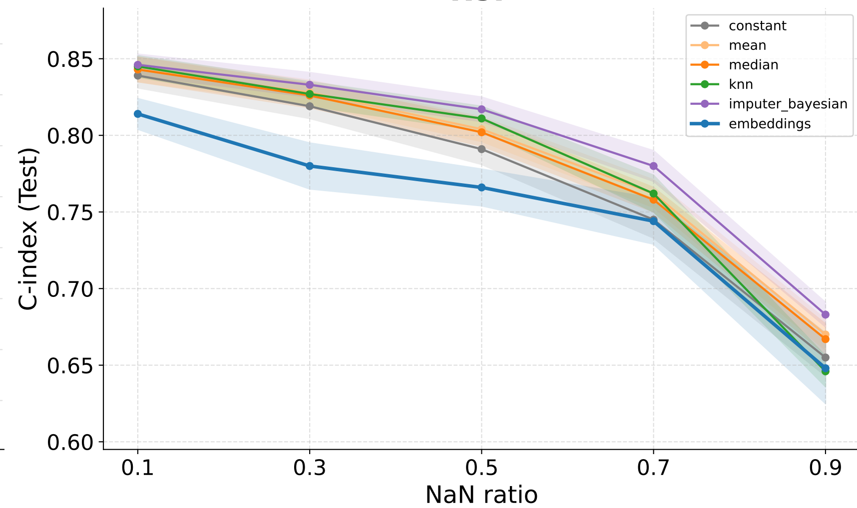
RSF
