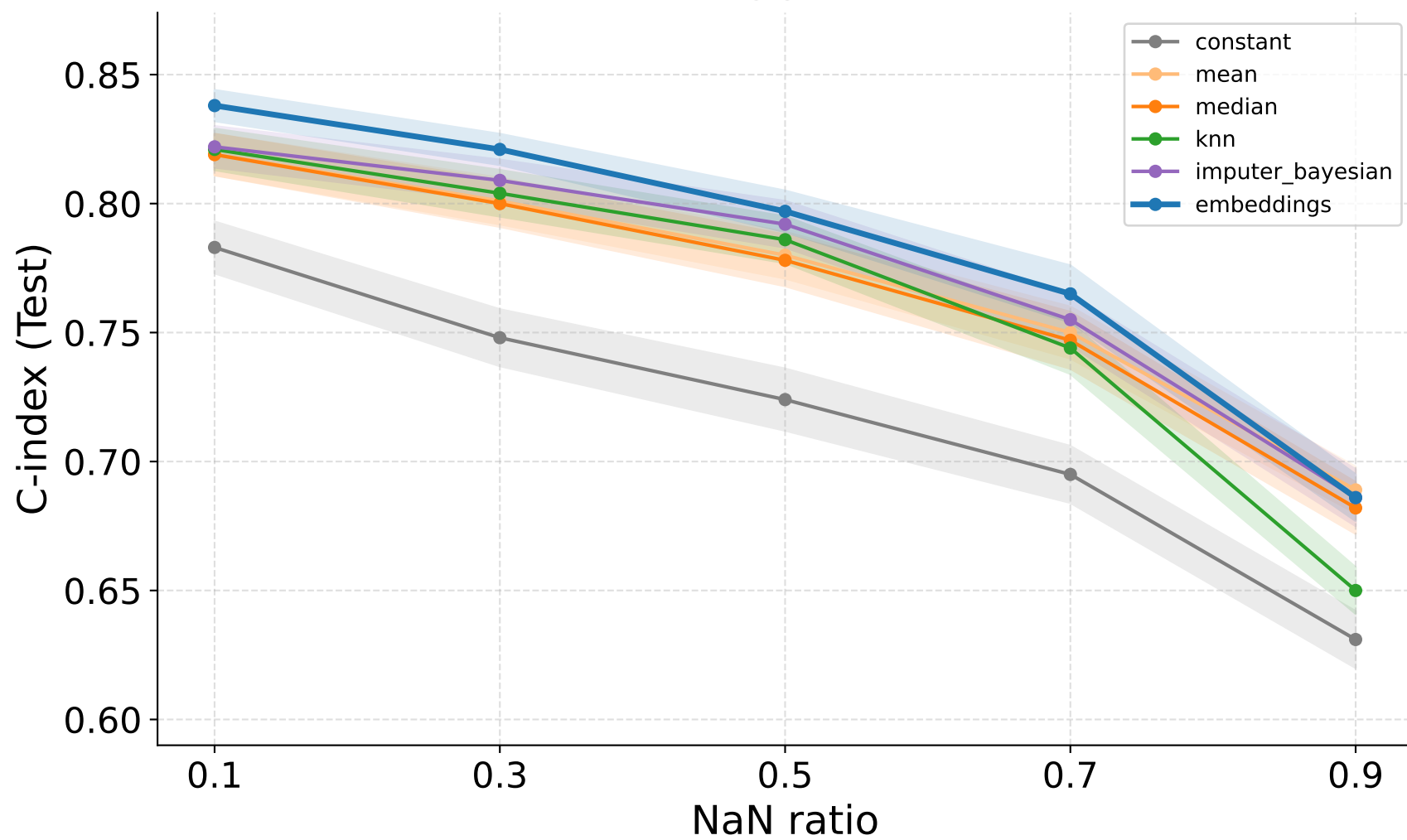
DeepSurv MLP
