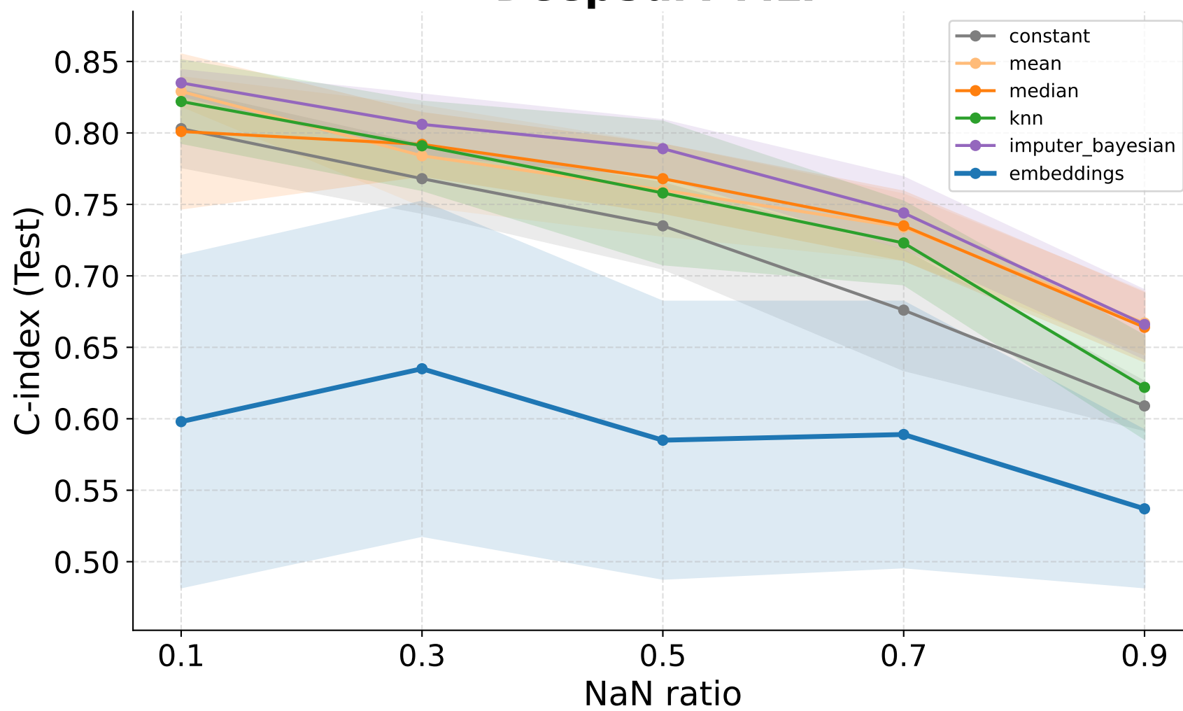
DeepSurv MLP
