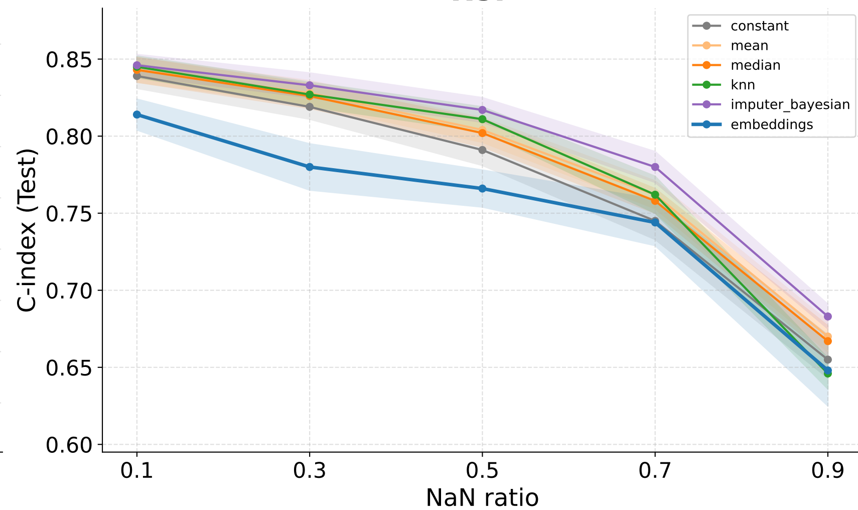
RSF
