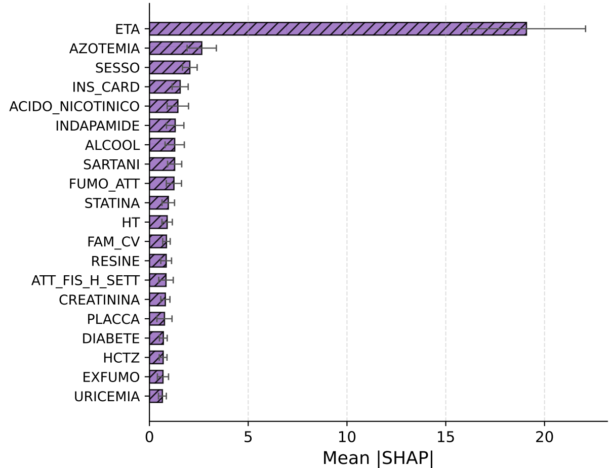
TabPFN - RSF tuned
