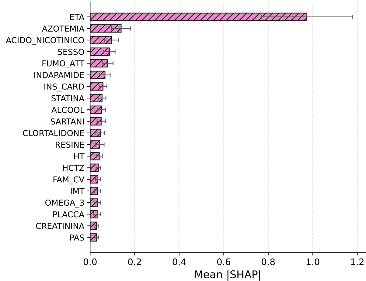
TabPFN - DeepSurv Linear
