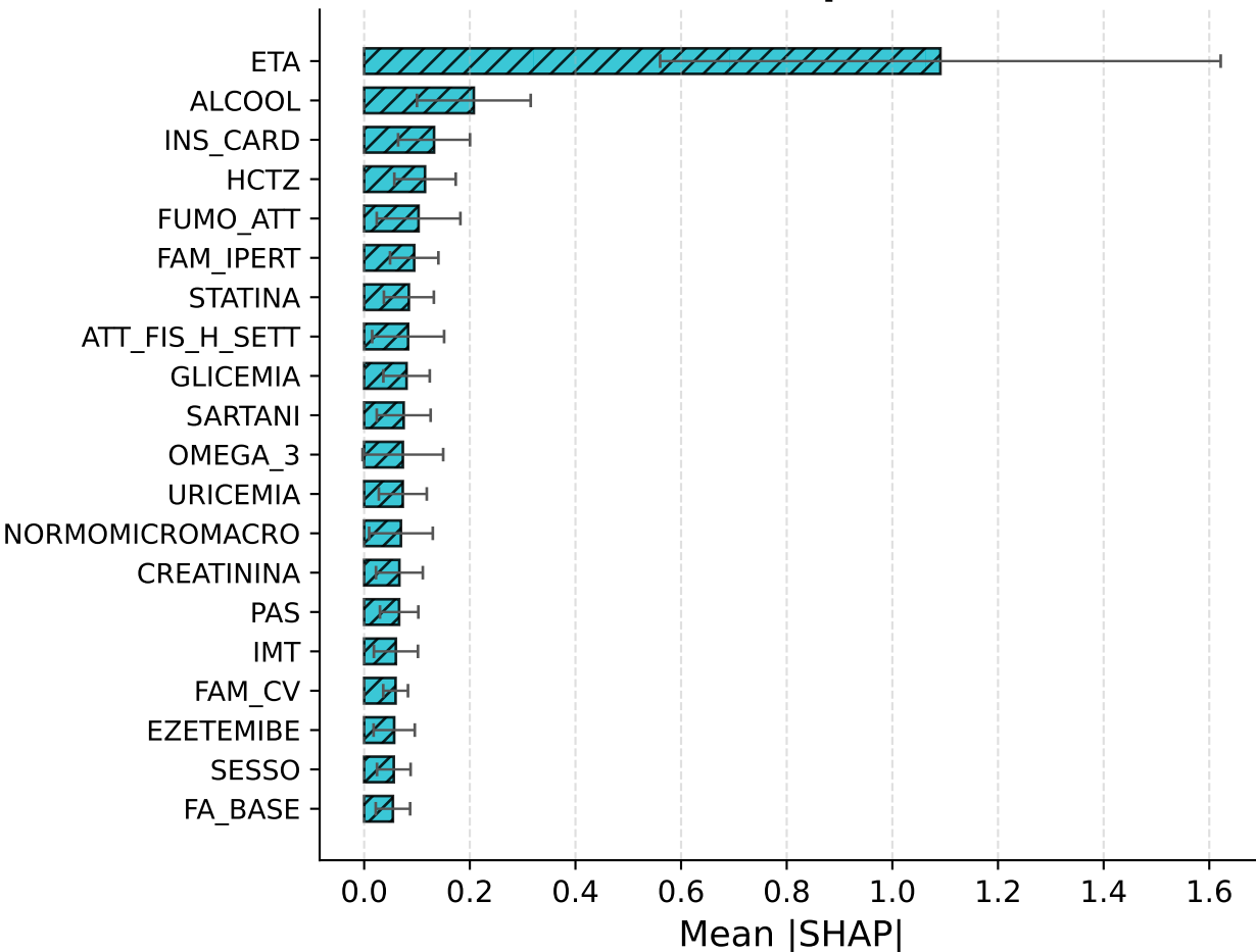
TabPFN - DeepSurv MLP
