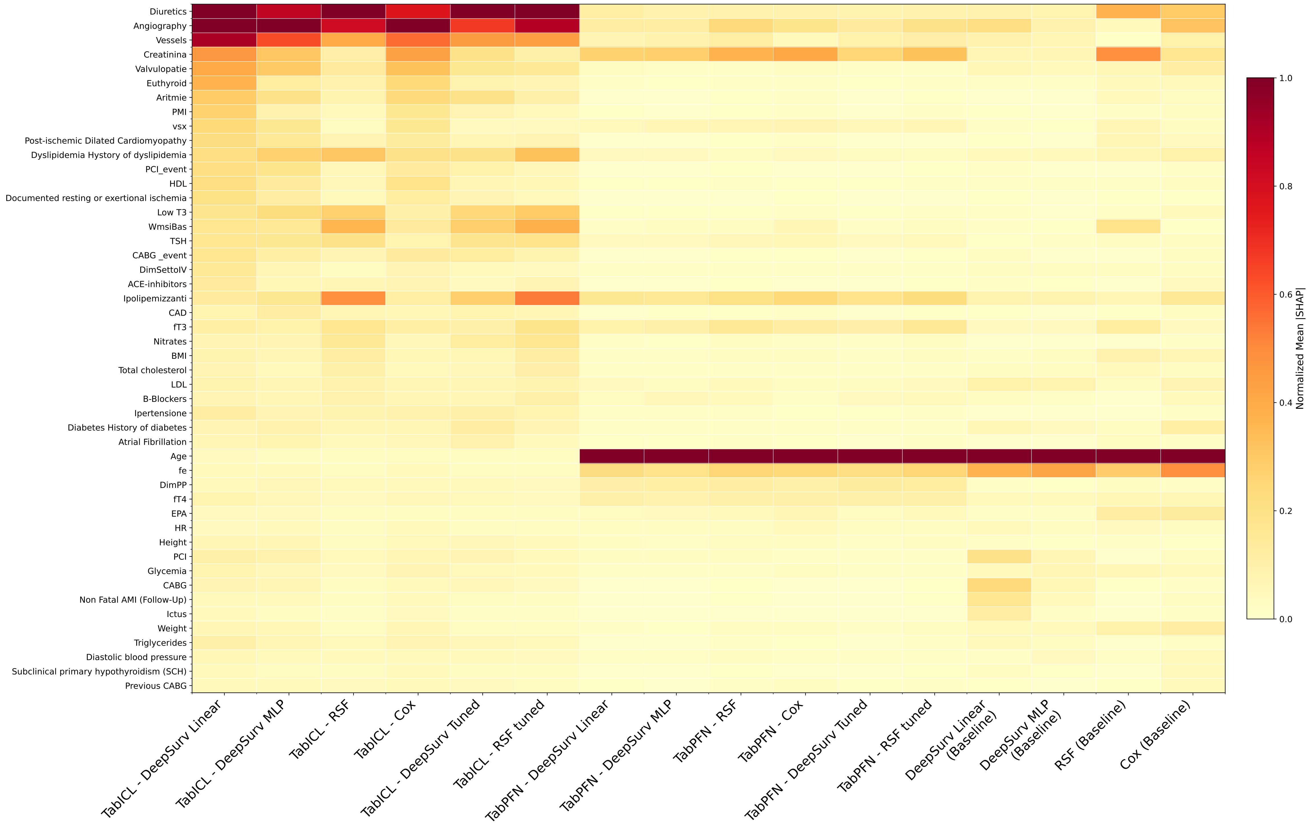
SHAP Feature Importance — IHD | TabICL + TabPFN | Preprocessing: -1 Top 20 features per model, normalized per model
