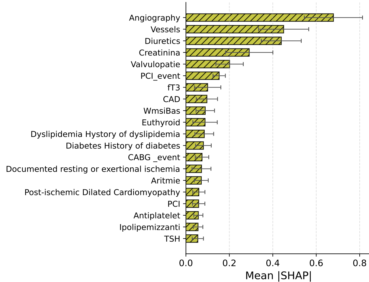
TabICL - Cox
