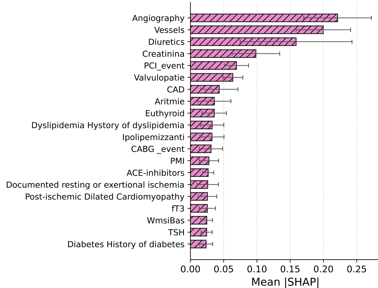
TabICL - Cox
