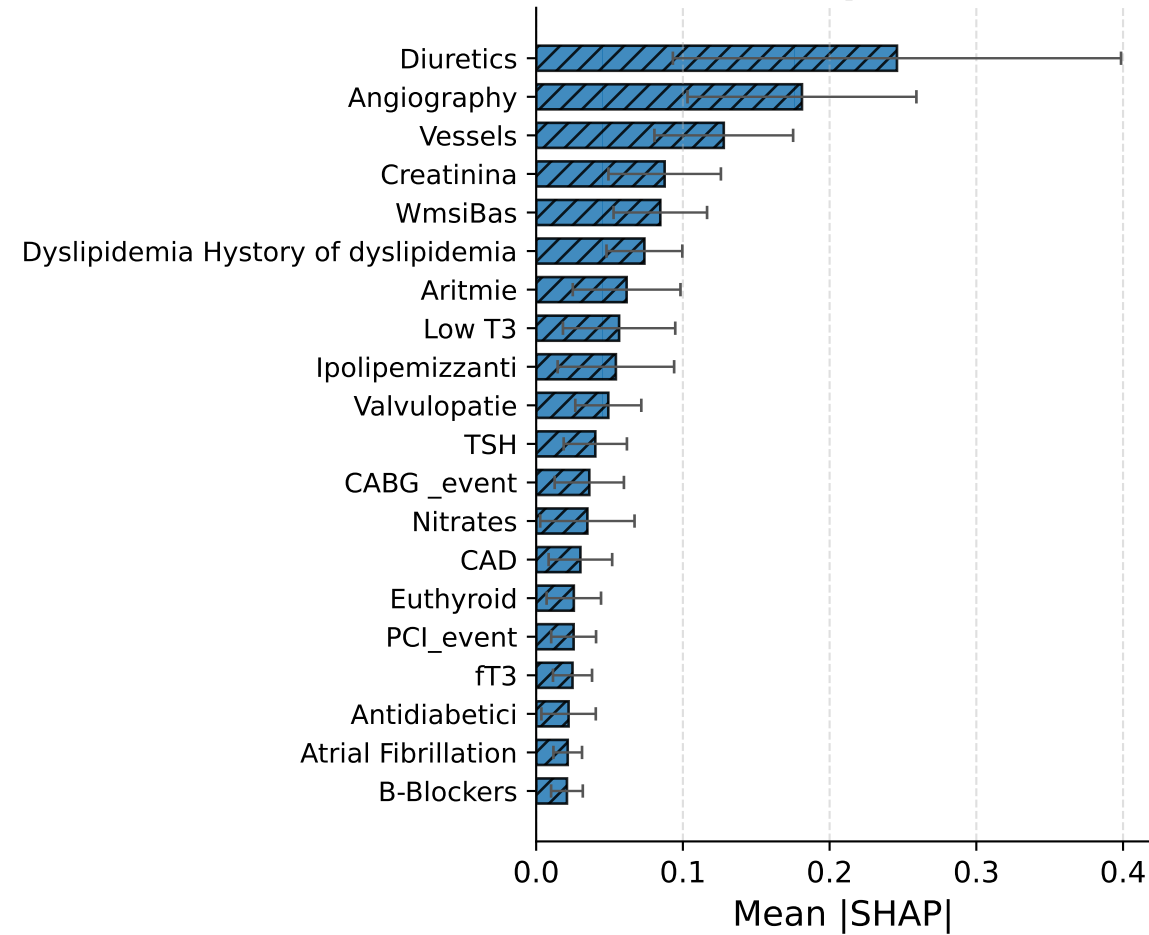
TabICL - DeepSurv Tuned
