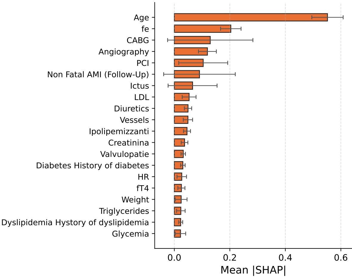
DeepSurv Linear (Baseline)
