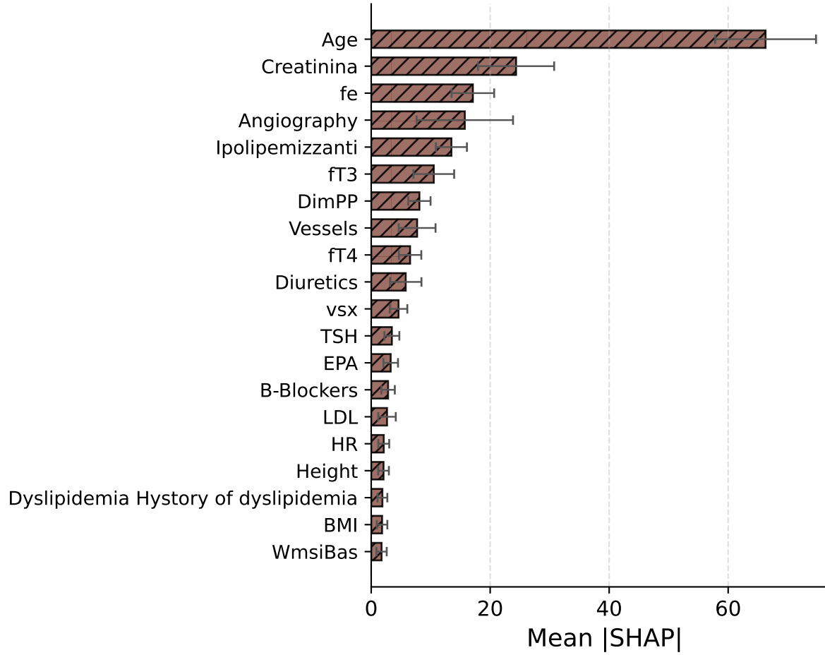
TabPFN - RSF
