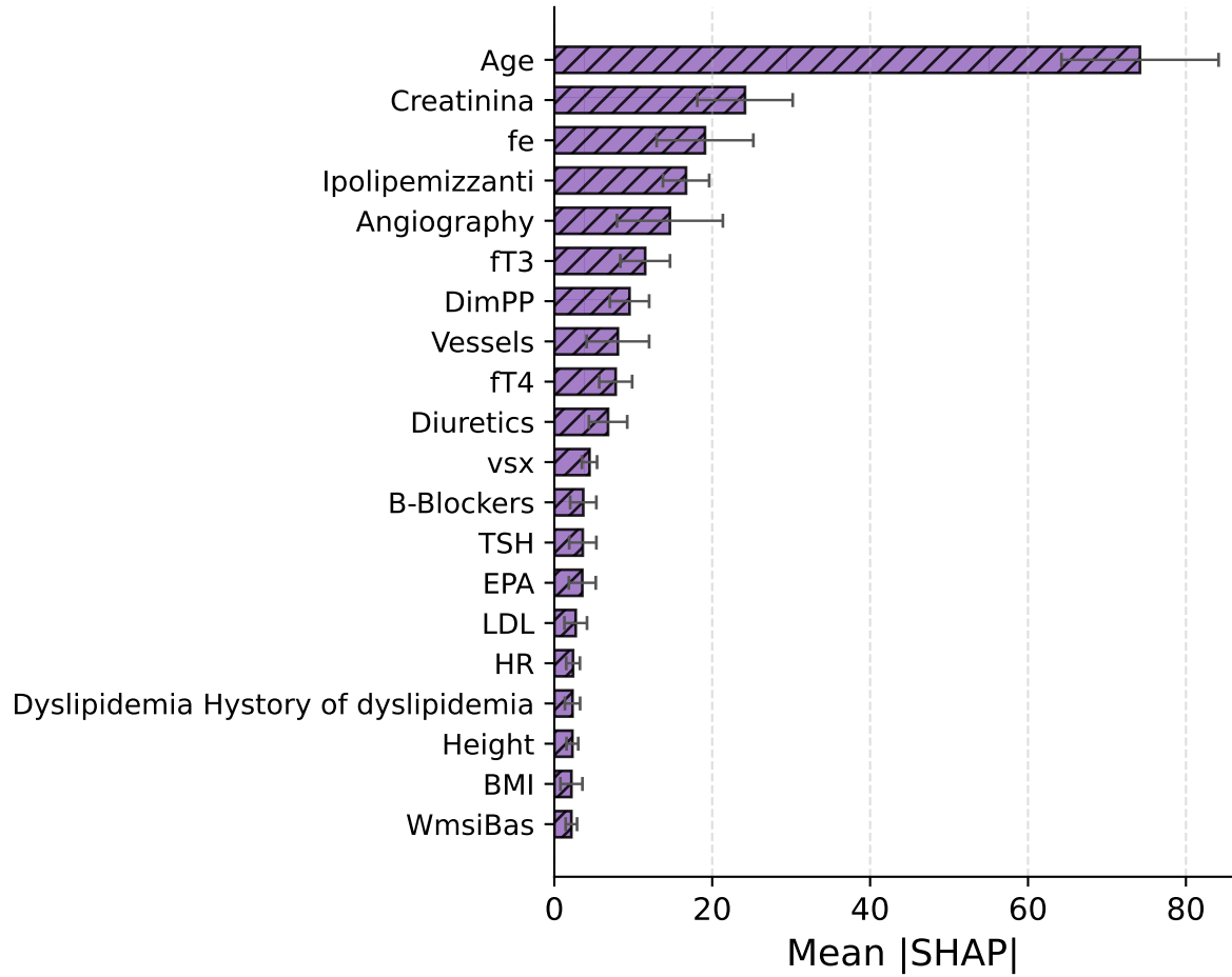
TabPFN - RSF tuned
