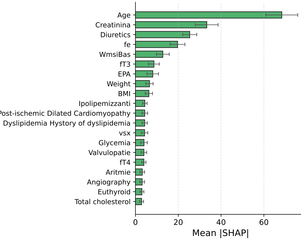
RSF (Baseline)
