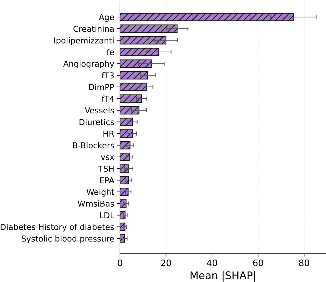
TabPFN - RSF tuned
