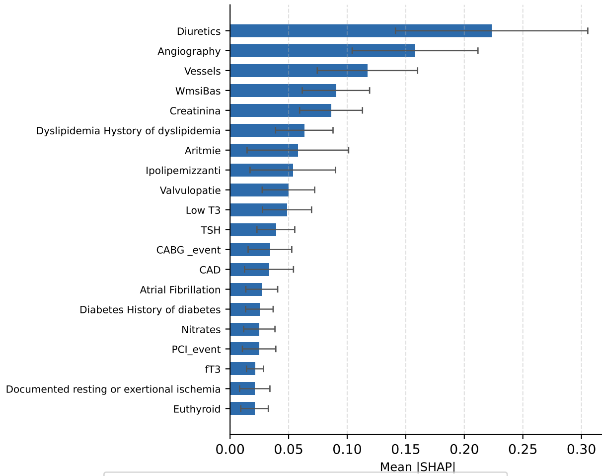
DeepSurv Tuned
