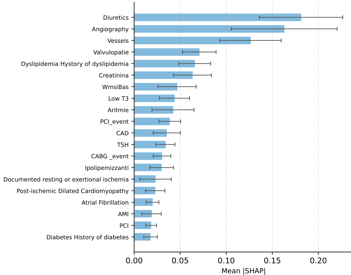
DeepSurv Tuned
