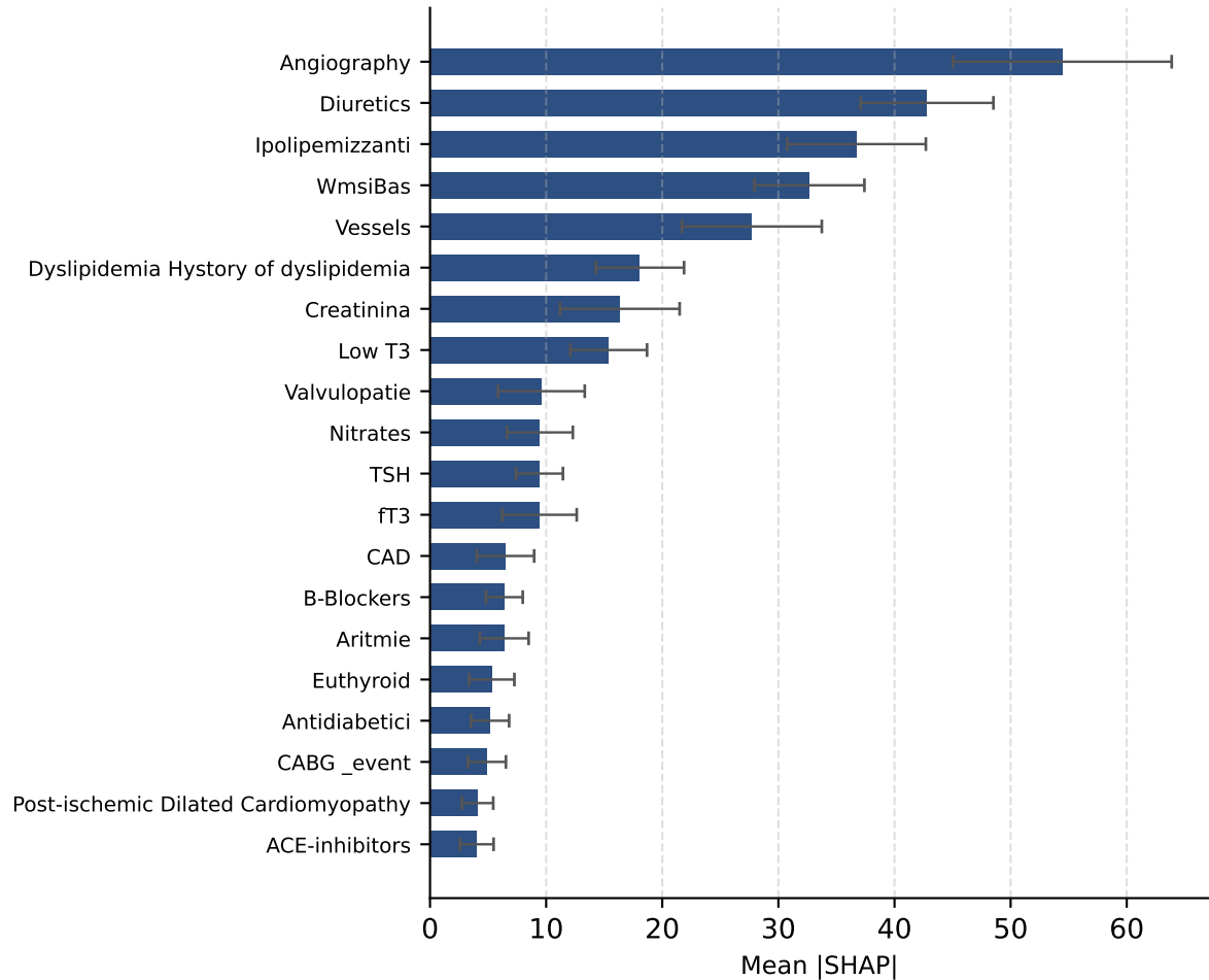
RSF
