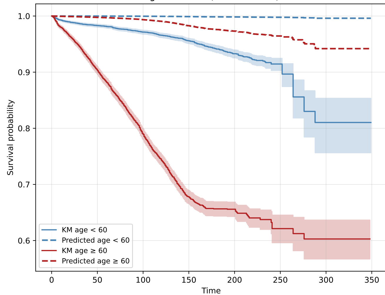
Age-stratified (< 60 vs \geq 60 )
