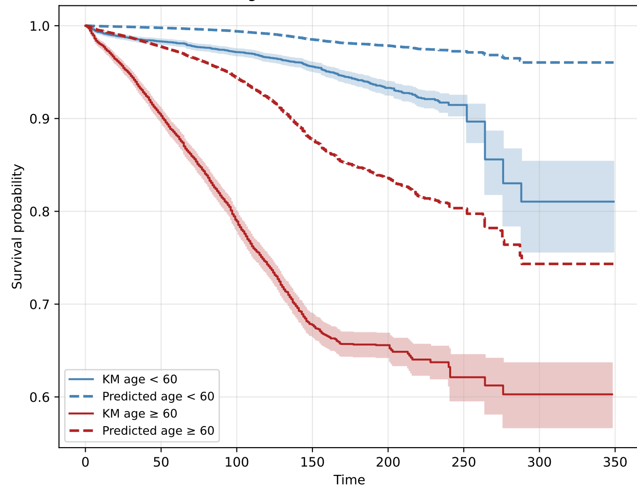
Age-stratified (&lt; 60 vs ≥ 60)
