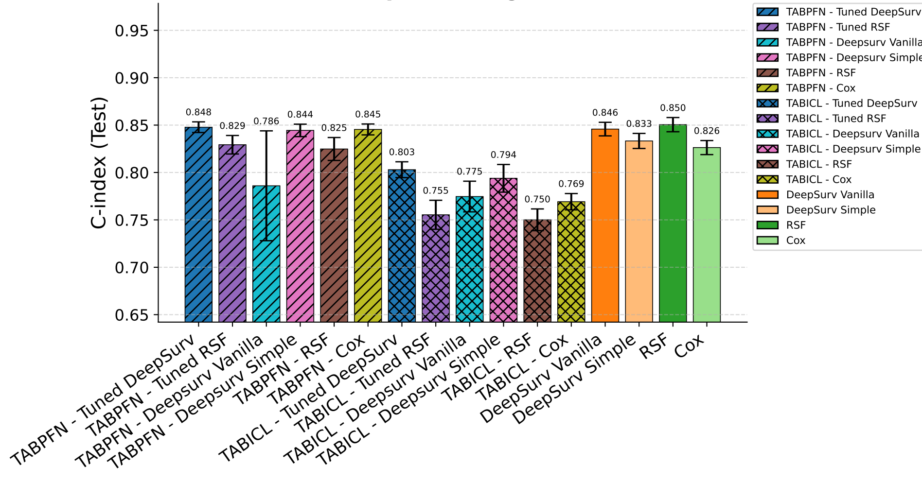
Preprocessing: -1
