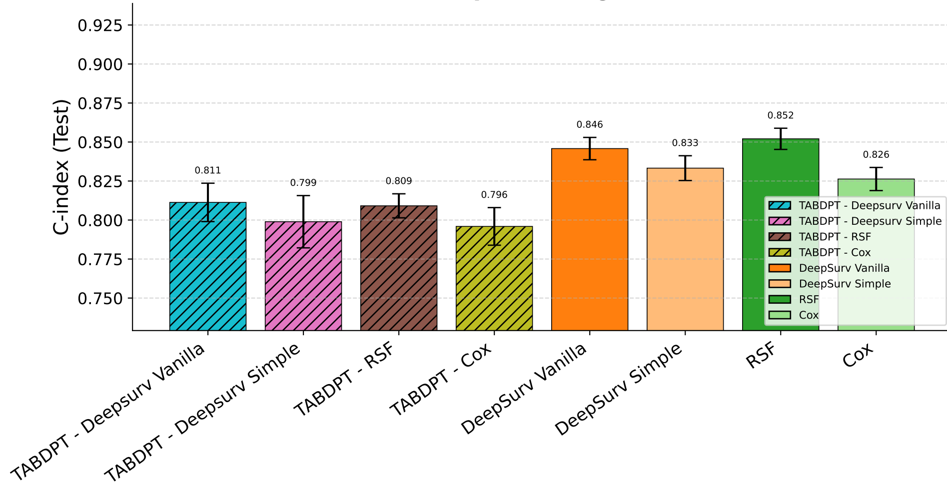
Preprocessing: -1
