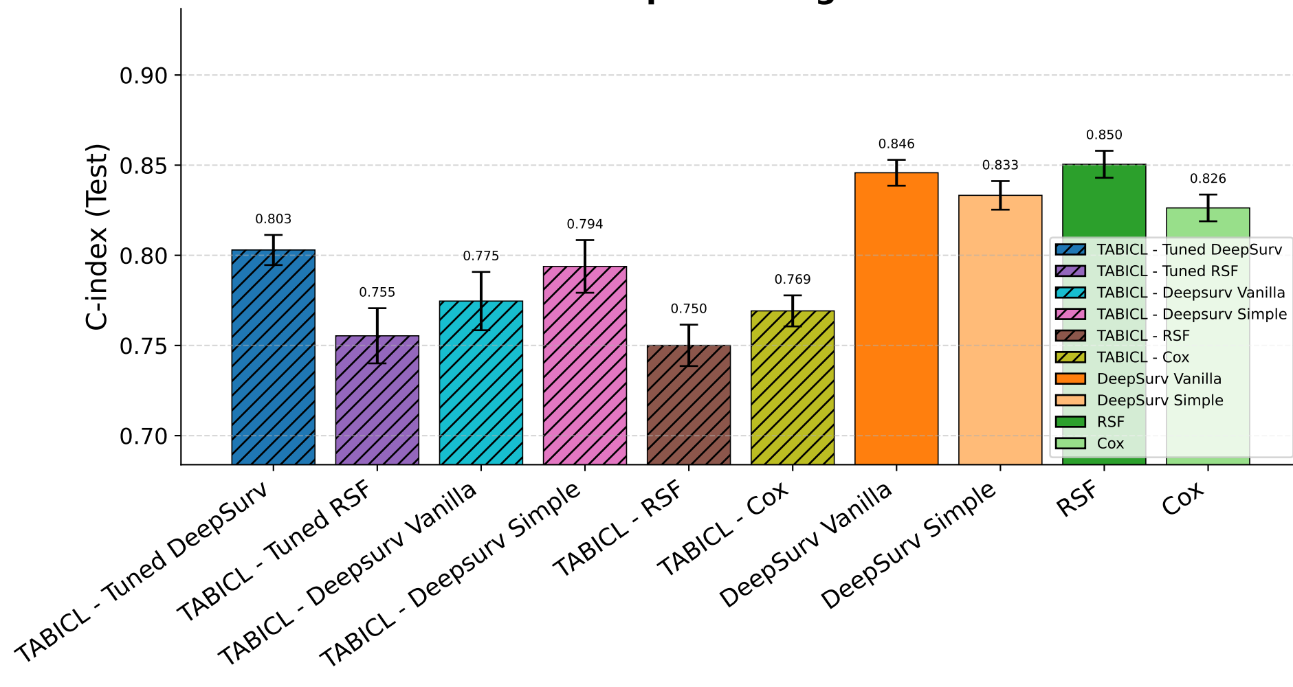
Preprocessing: -1
