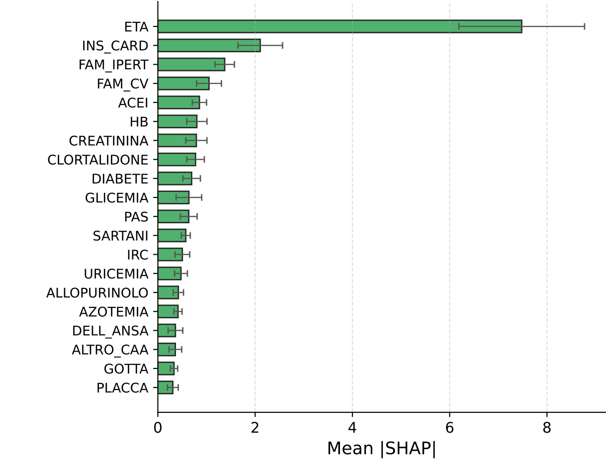
RSF (Baseline)
