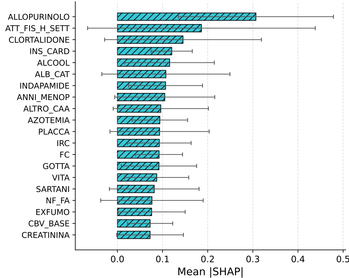
DeepSurv MLP
