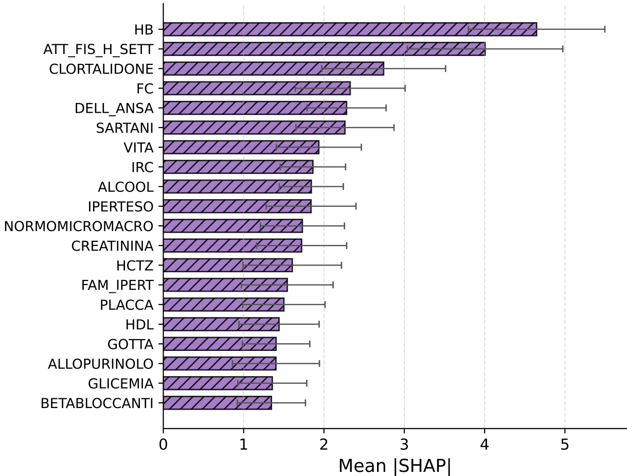
RSF tuned
