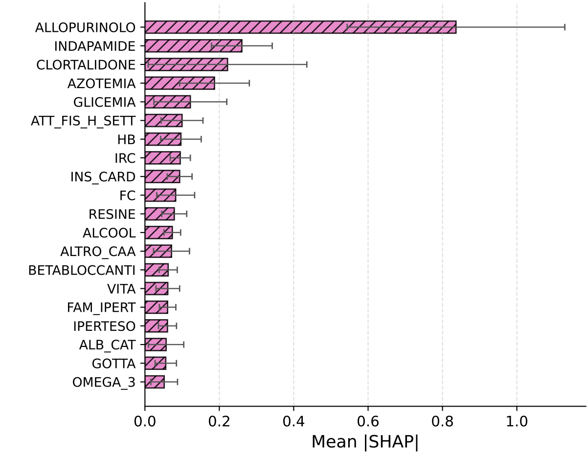
DeepSurv Linear
