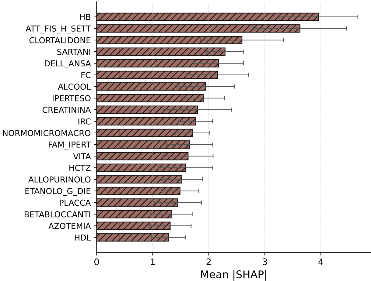
RSF
