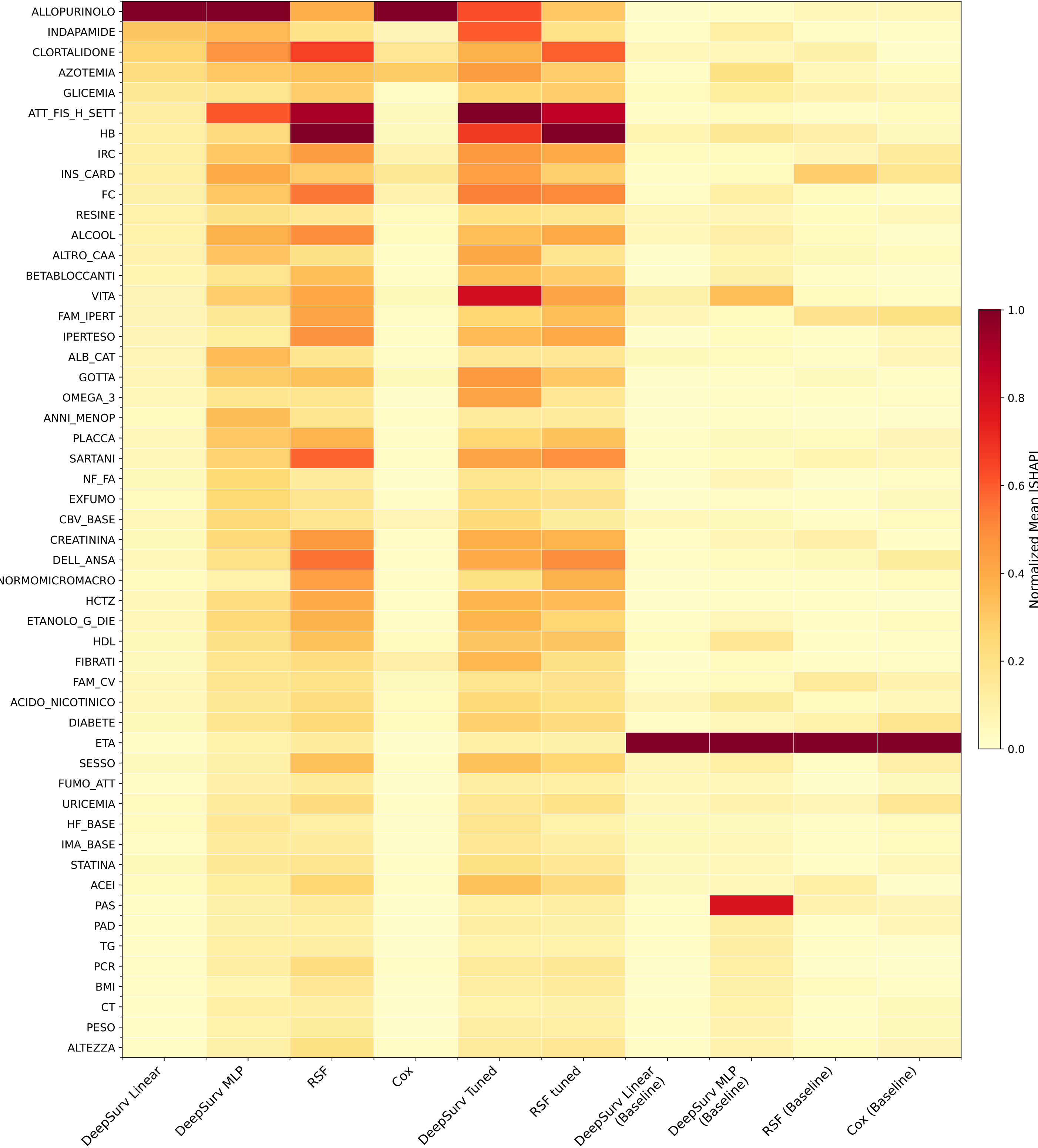
SHAP Feature Importance — URRAH | tabicl | Preprocessing: -1 Top 20 features per model, normalized per model
