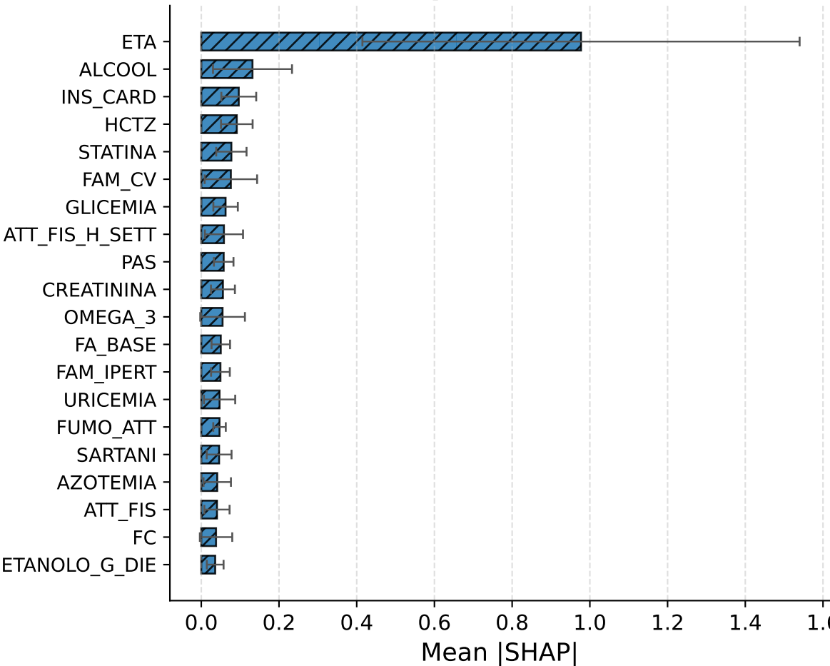
DeepSurv Tuned
