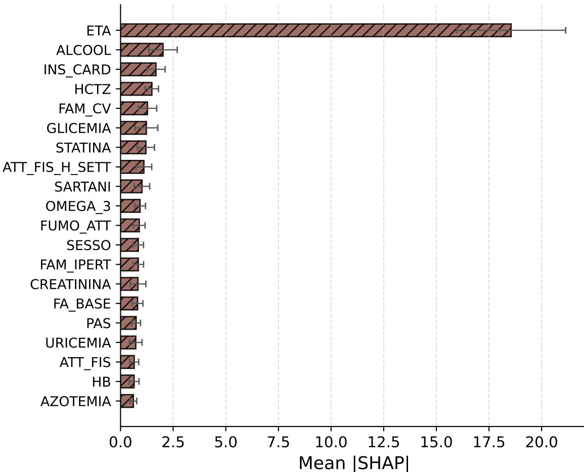
RSF
