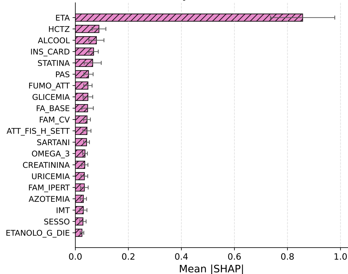
DeepSurv Linear
