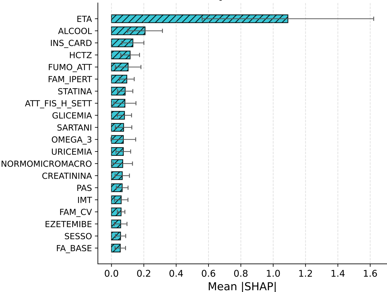
DeepSurv MLP
