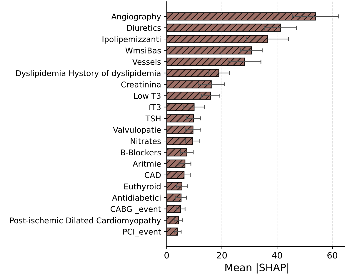
RSF tuned
