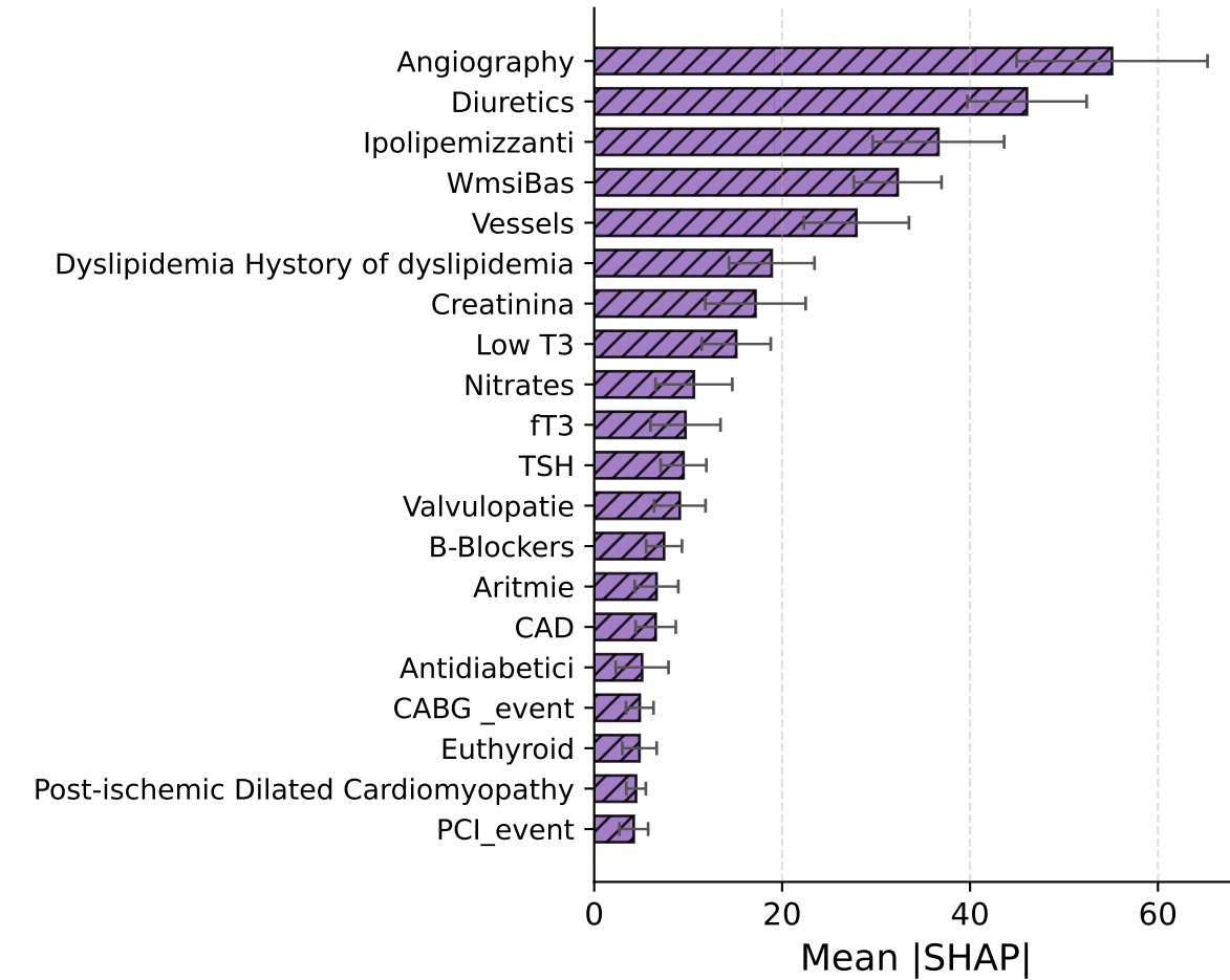
RSF tuned
