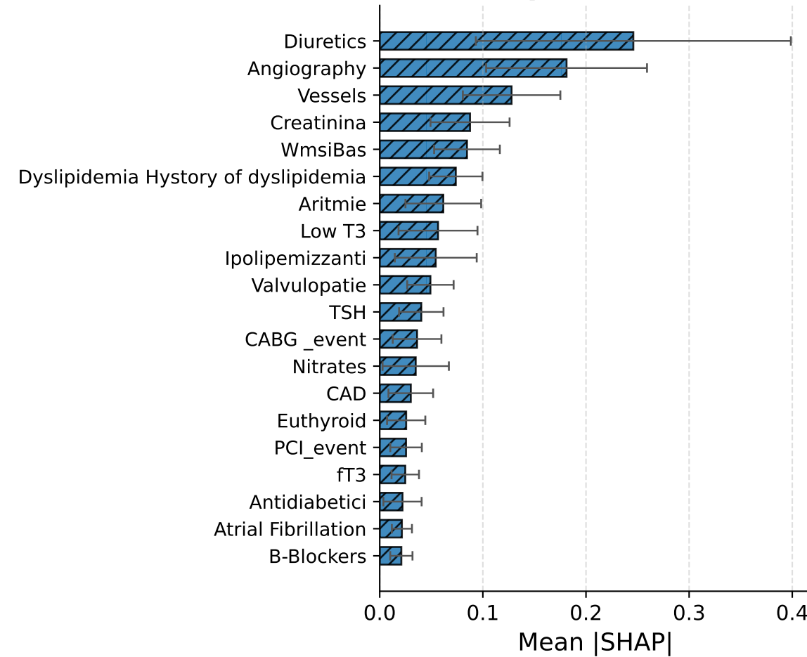
DeepSurv Tuned
