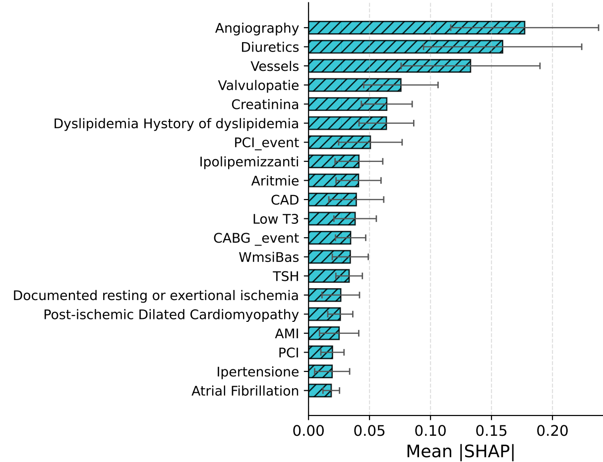
DeepSurv Tuned
