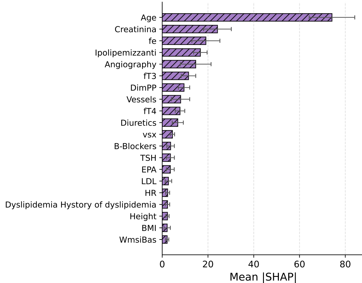
RSF tuned
