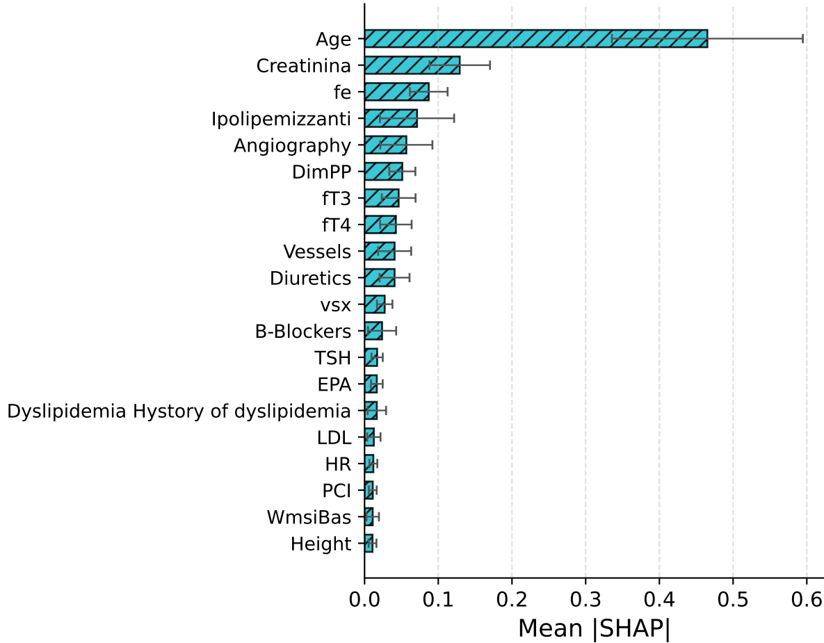
DeepSurv MLP
