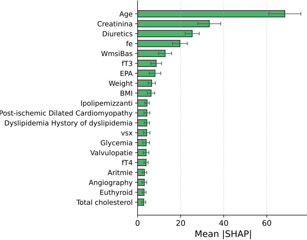
RSF (Baseline)
