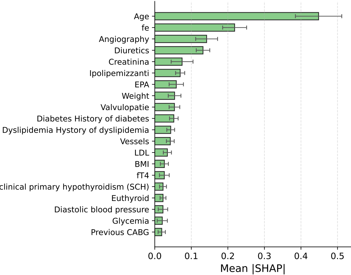
Cox (Baseline)
