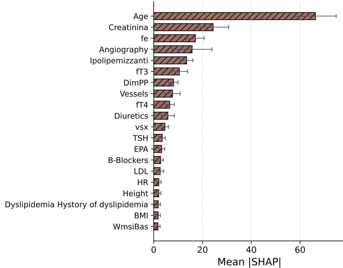
RSF
