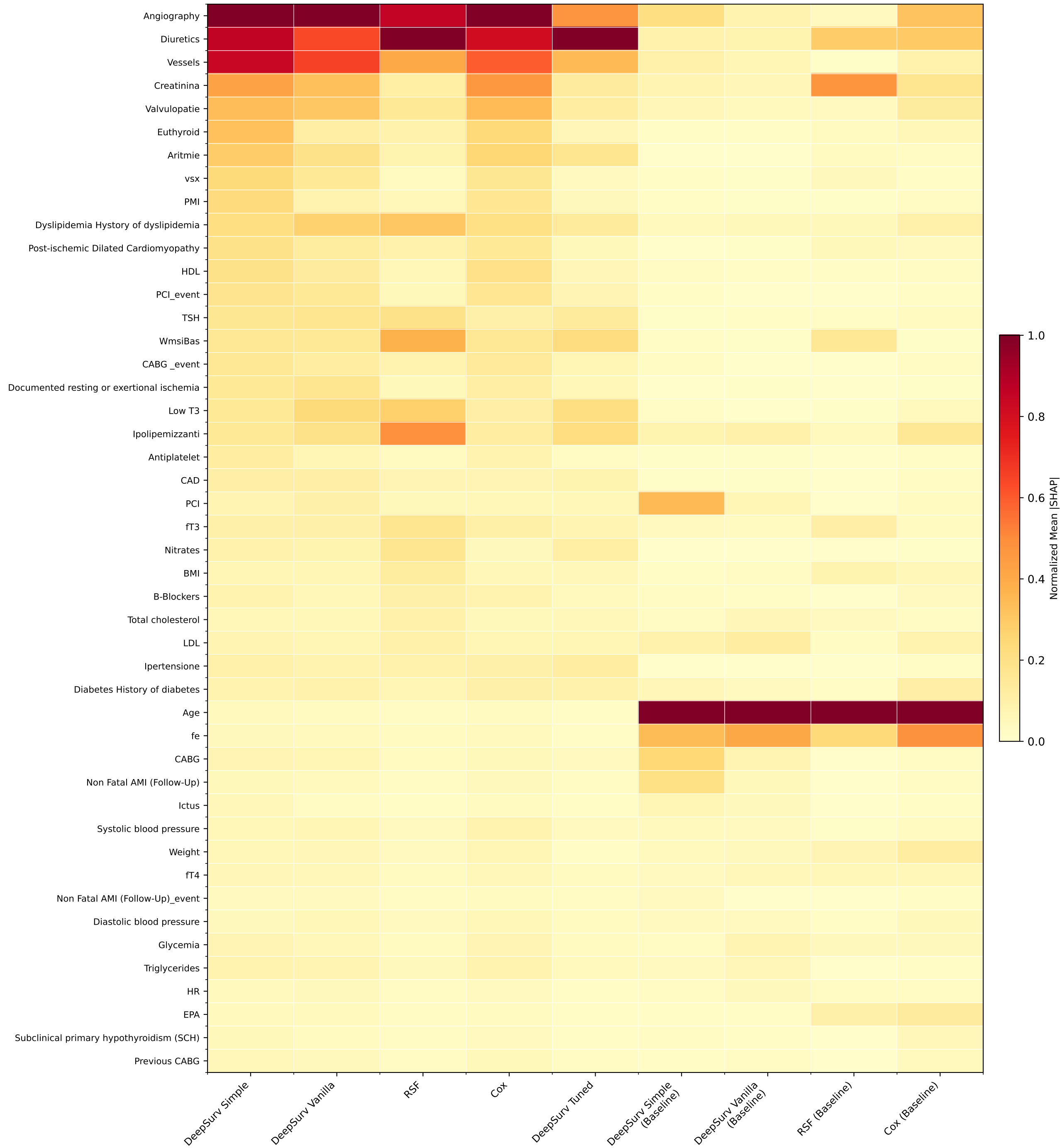
SHAP Feature Importance — OrmoniTirodei | tabicl | Preprocessing: -1 Top 20 features per model, normalized per model
