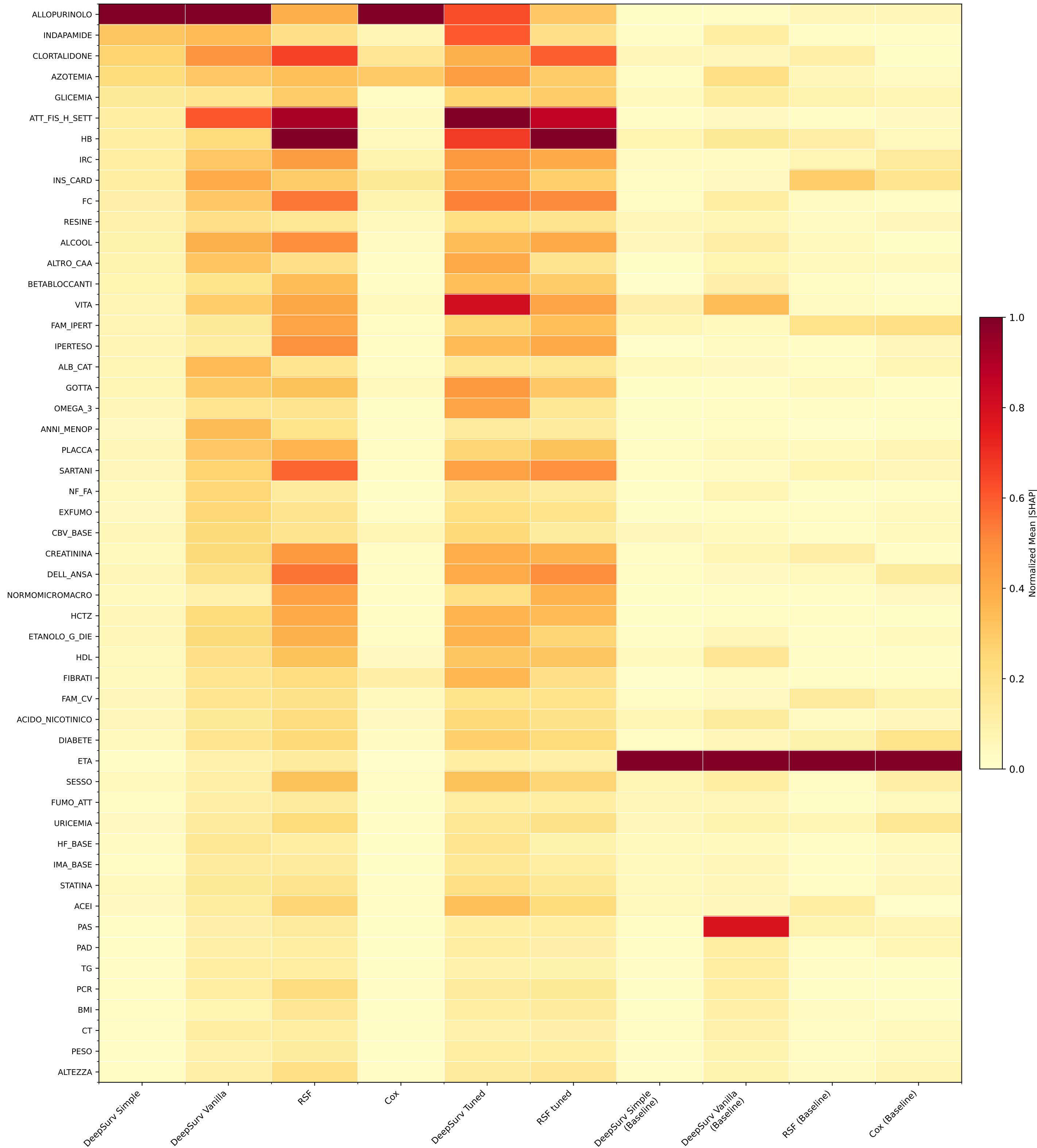
SHAP Feature Importance — URRAH | tabici | Preprocessing: -1 Top 20 features per model, normalized per model
