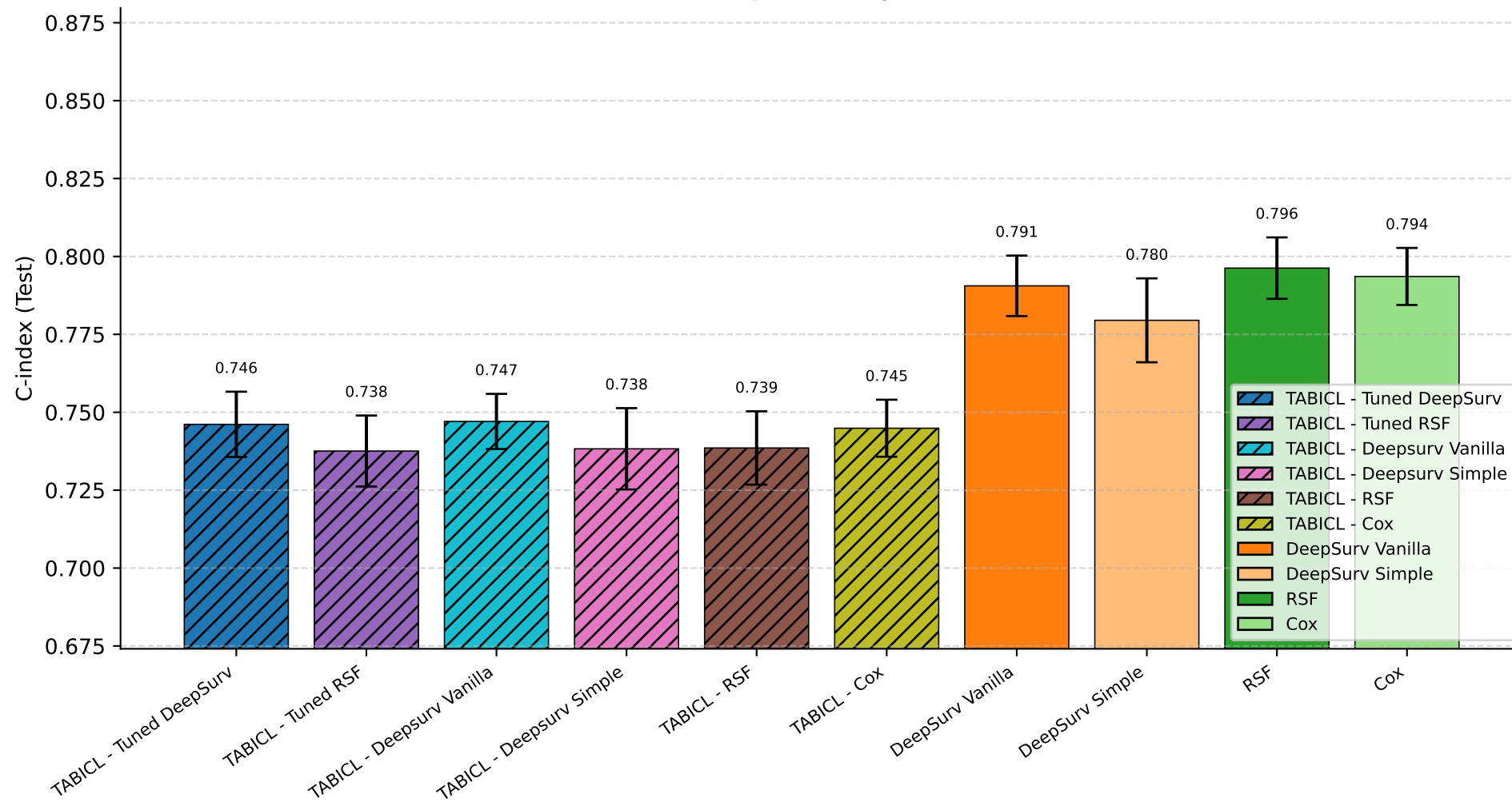
Preprocessing: -1
