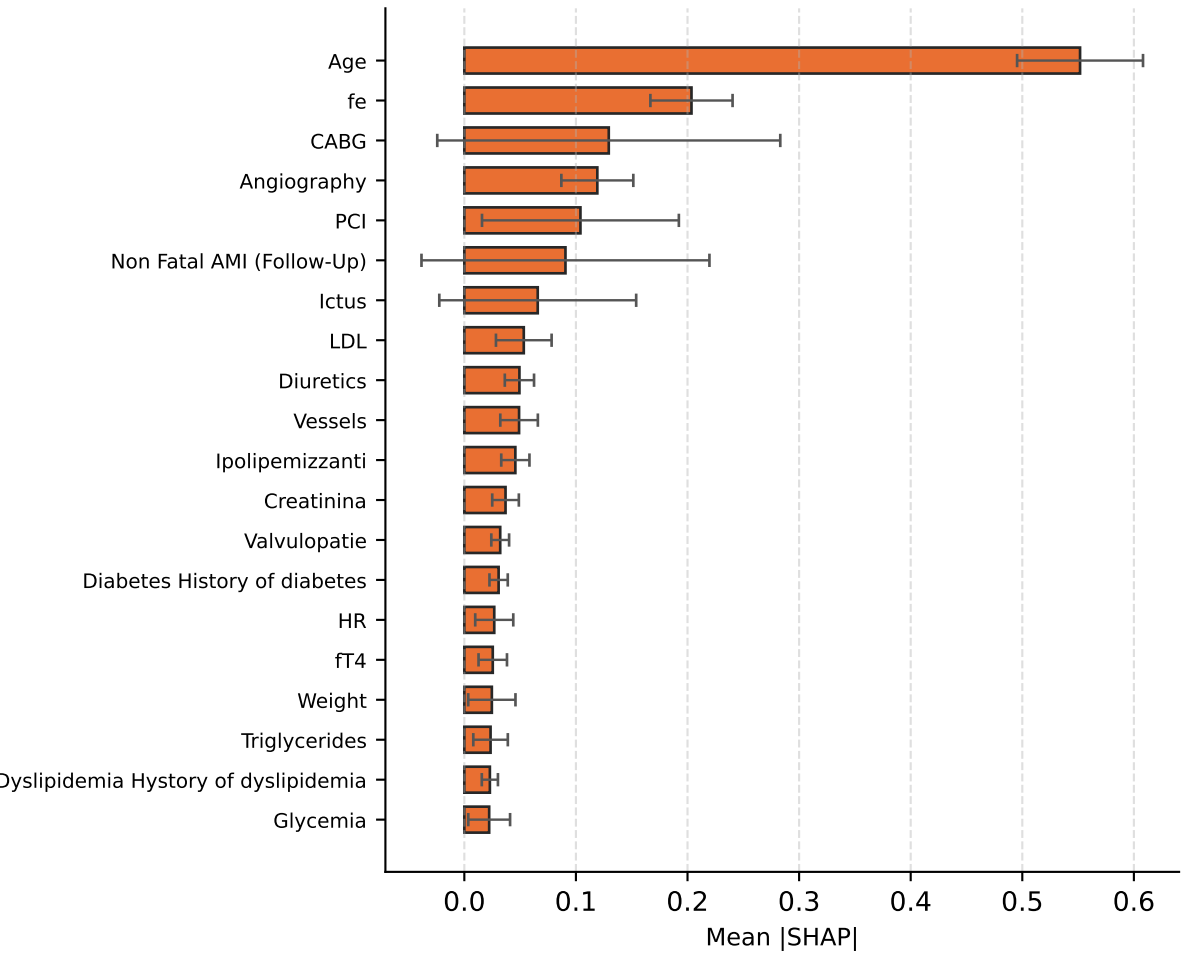
DeepSurv Simple (Baseline)
