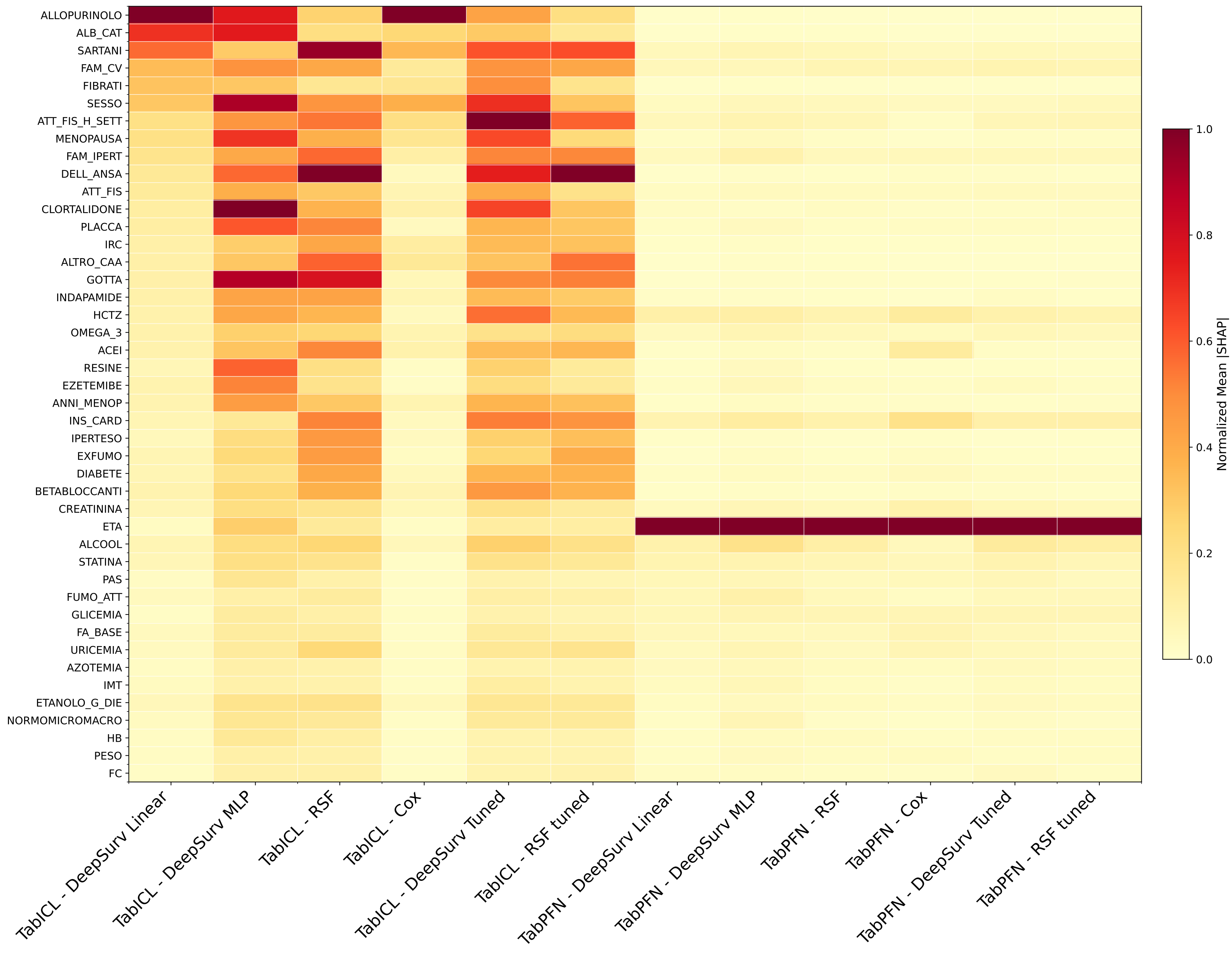
SHAP Feature Importance — URRAH | TabICL + TabPFN | Preprocessing: NaN Top 20 features per model, normalized per model
