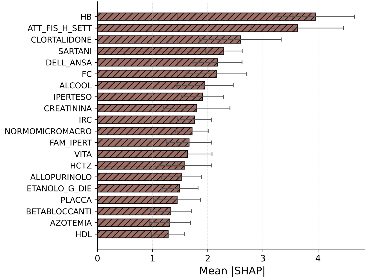
TabICL - RSF
