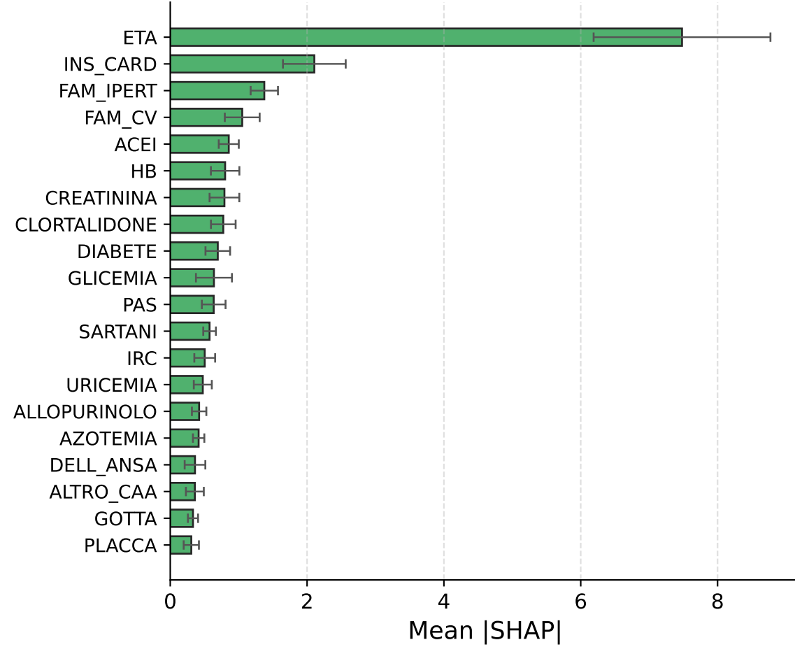
RSF (Baseline)
