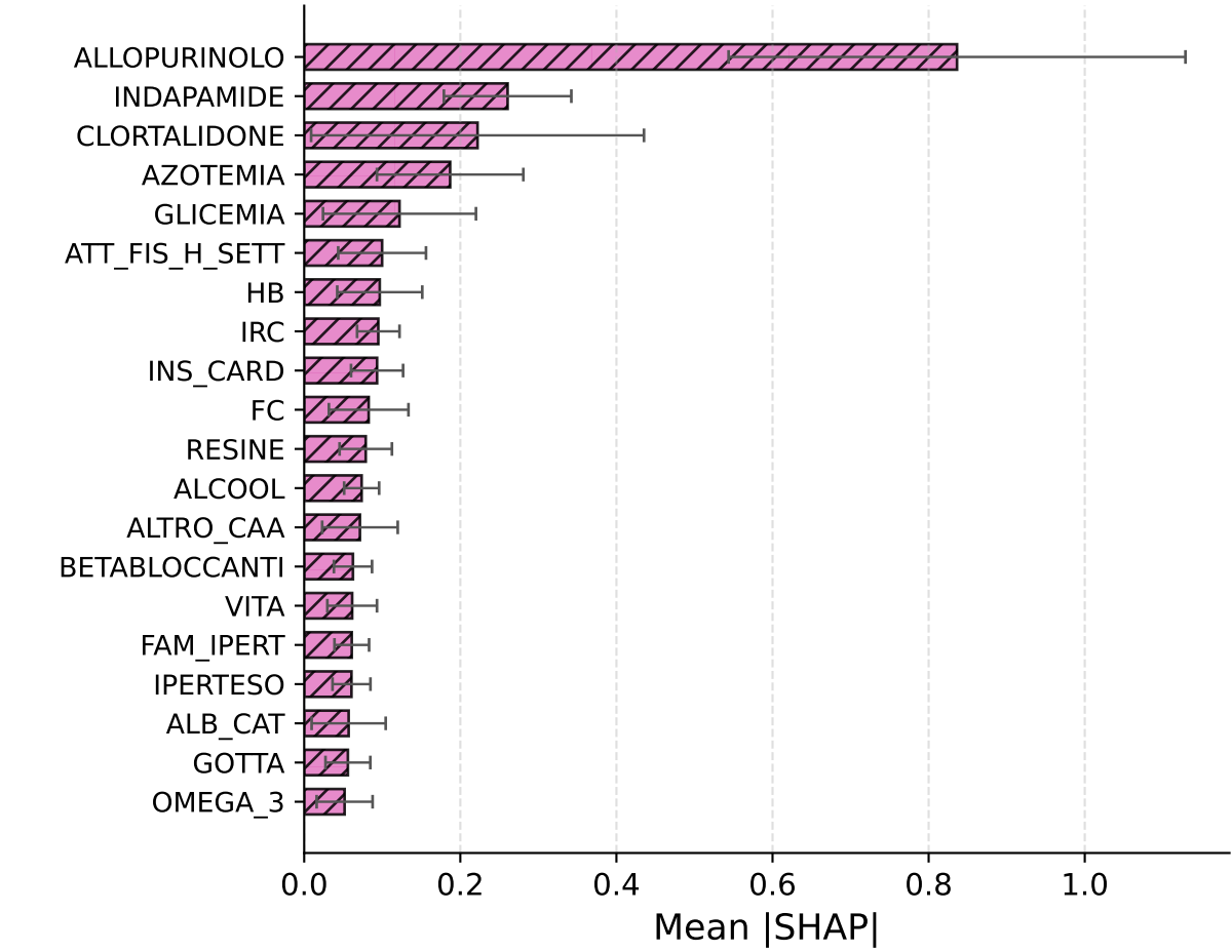
TabICL - DeepSurv Linear
