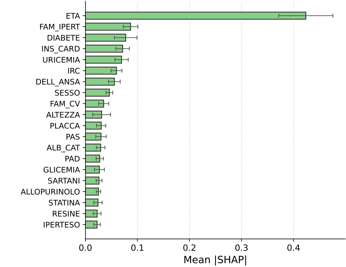
Cox (Baseline)
