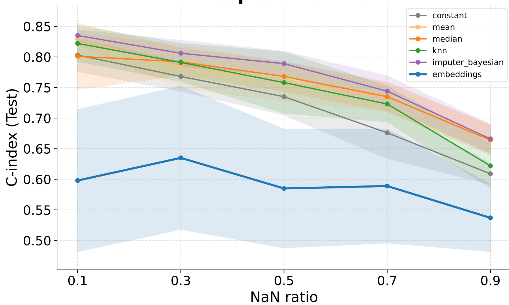
DeepSurv Vanilla
