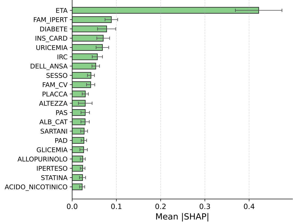
Cox (Baseline)
