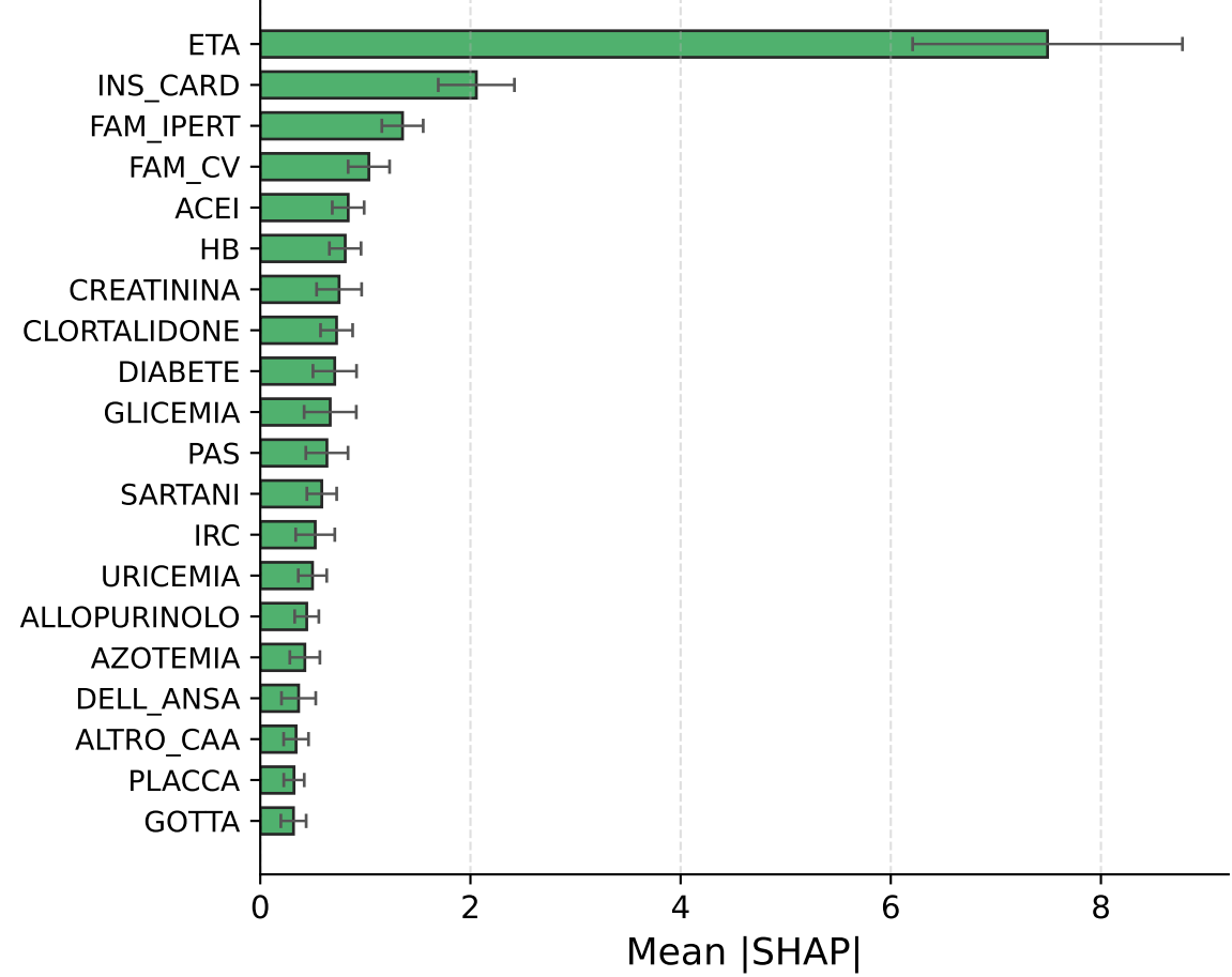
RSF (Baseline)
