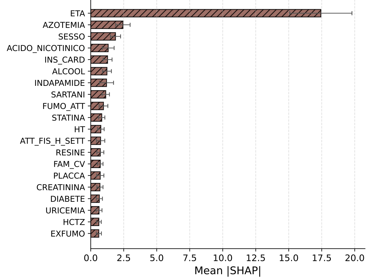
TabPFN - RSF
