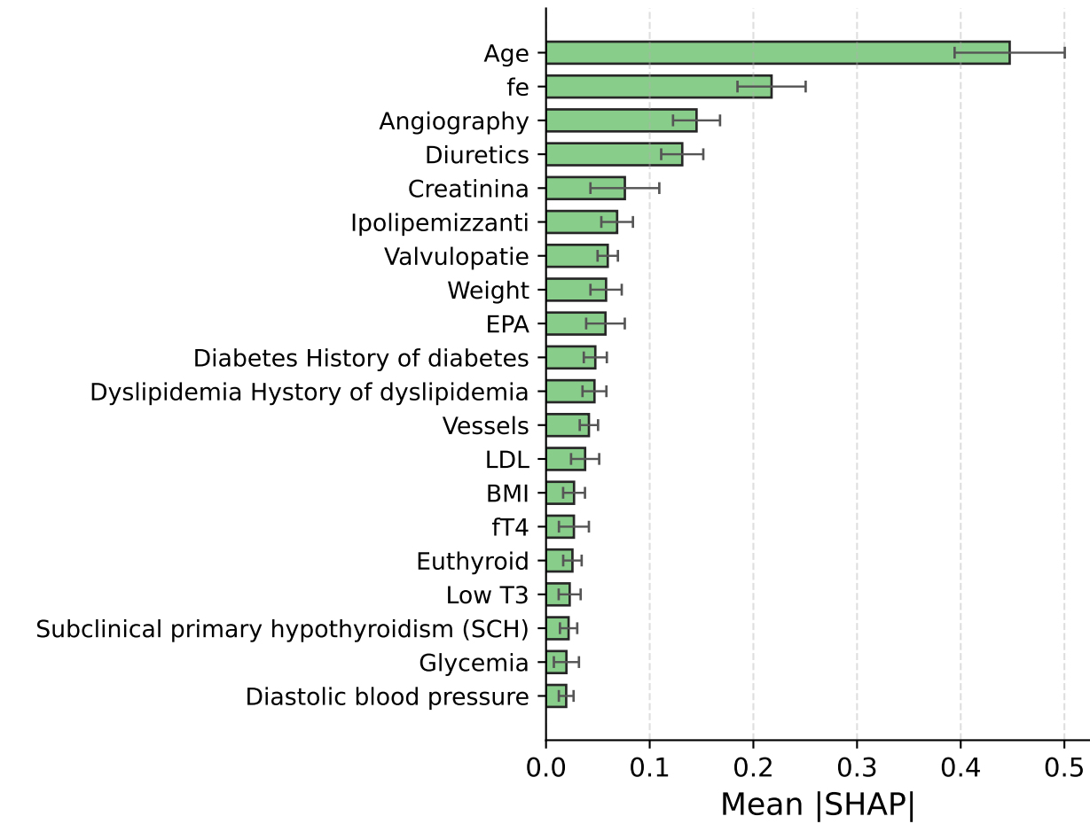
Cox (Baseline)
