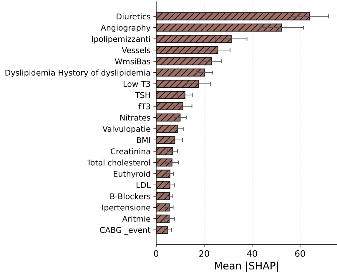
TabICL - RSF
