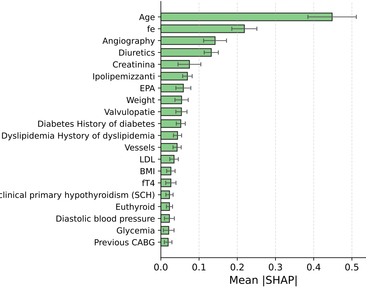
Cox (Baseline)
