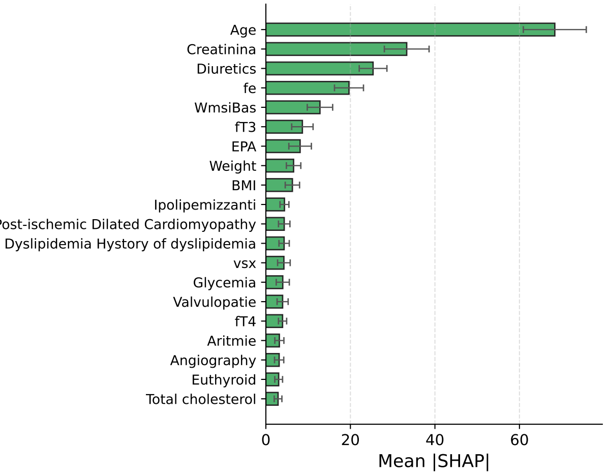
RSF (Baseline)
