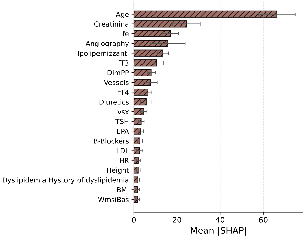
TabPFN - RSF
