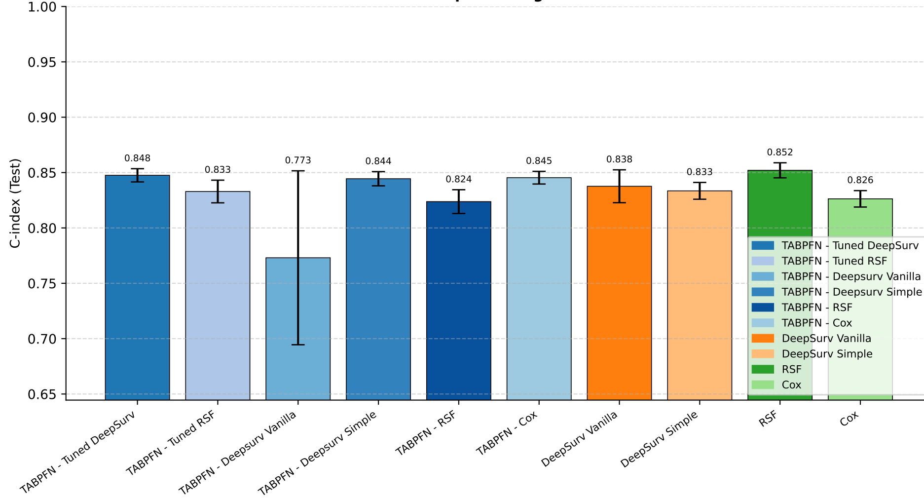
Preprocessing: -1
