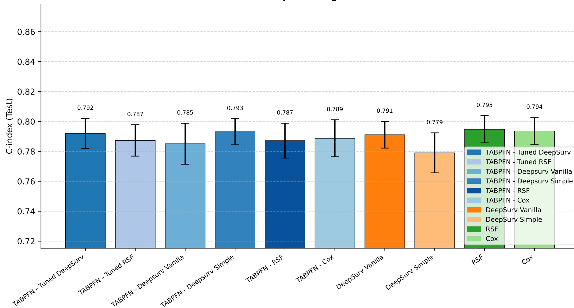
Preprocessing: -1
