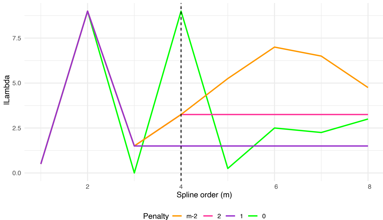
Comparison of LLAMBDA across penalties
