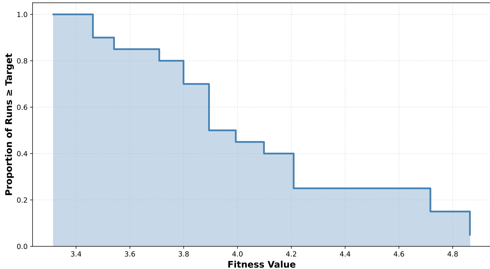
ECDF: F18 LABS (GA, D=50)
