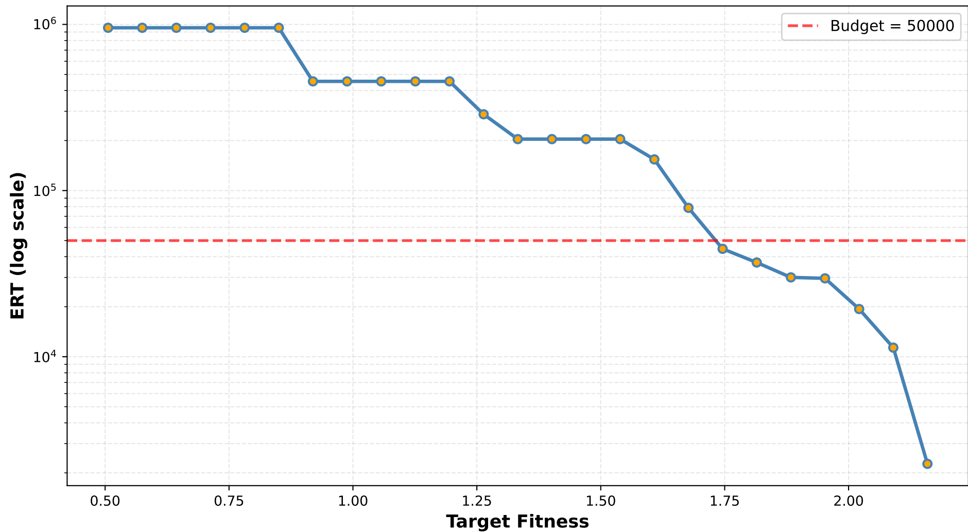
Expected Running Time: F23 Katsuura (ES, D=10)
