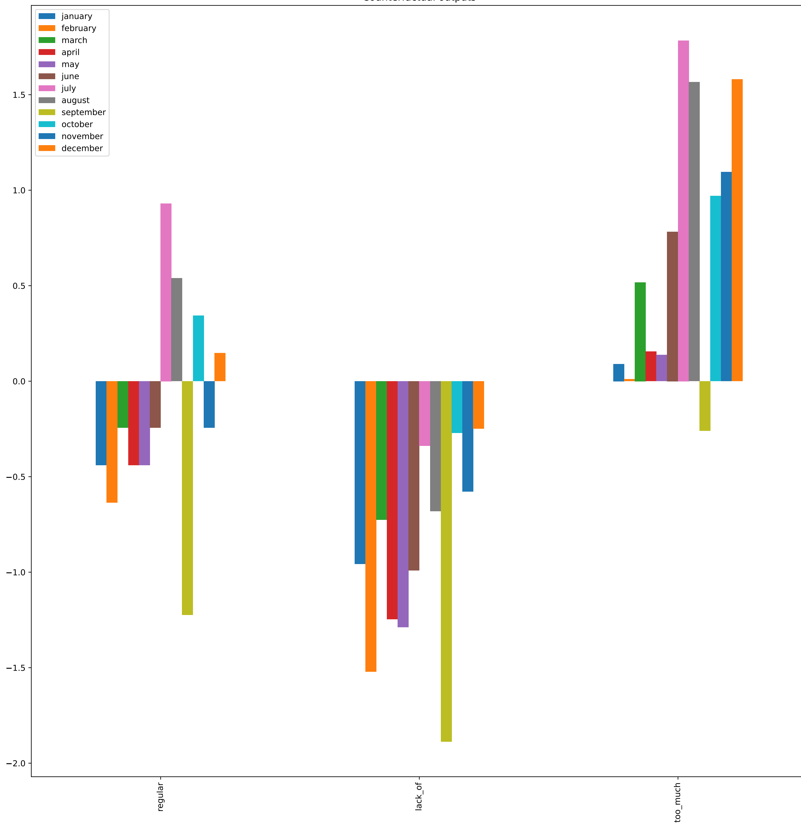
Counterfactual outputs
