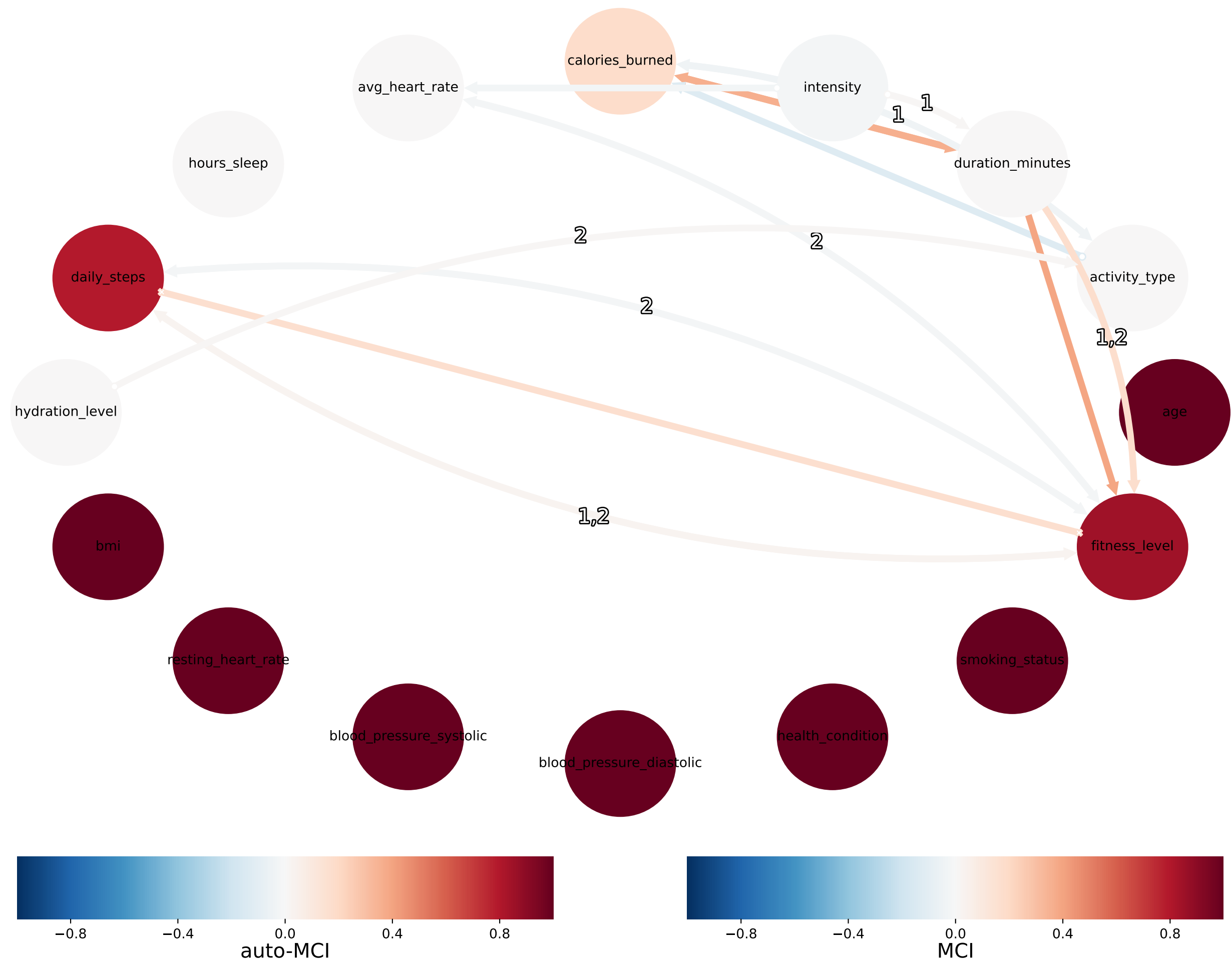
Causal discovery - LPCMCI with tau=2 pc=0.05 cit=PairwiseMultCI
