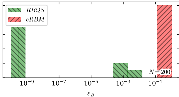
NQA (catalyzed)
