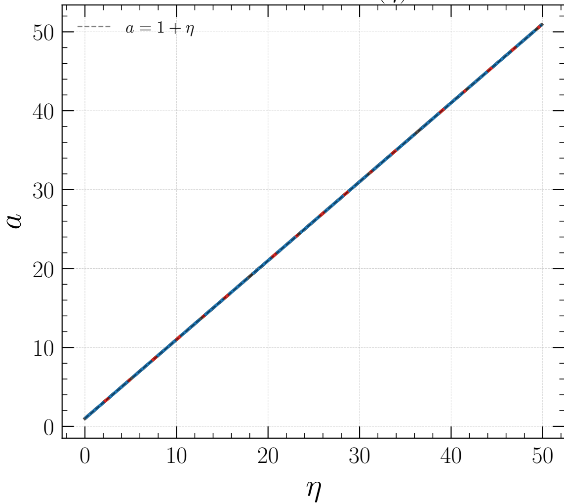
Scale factor a(\eta)
