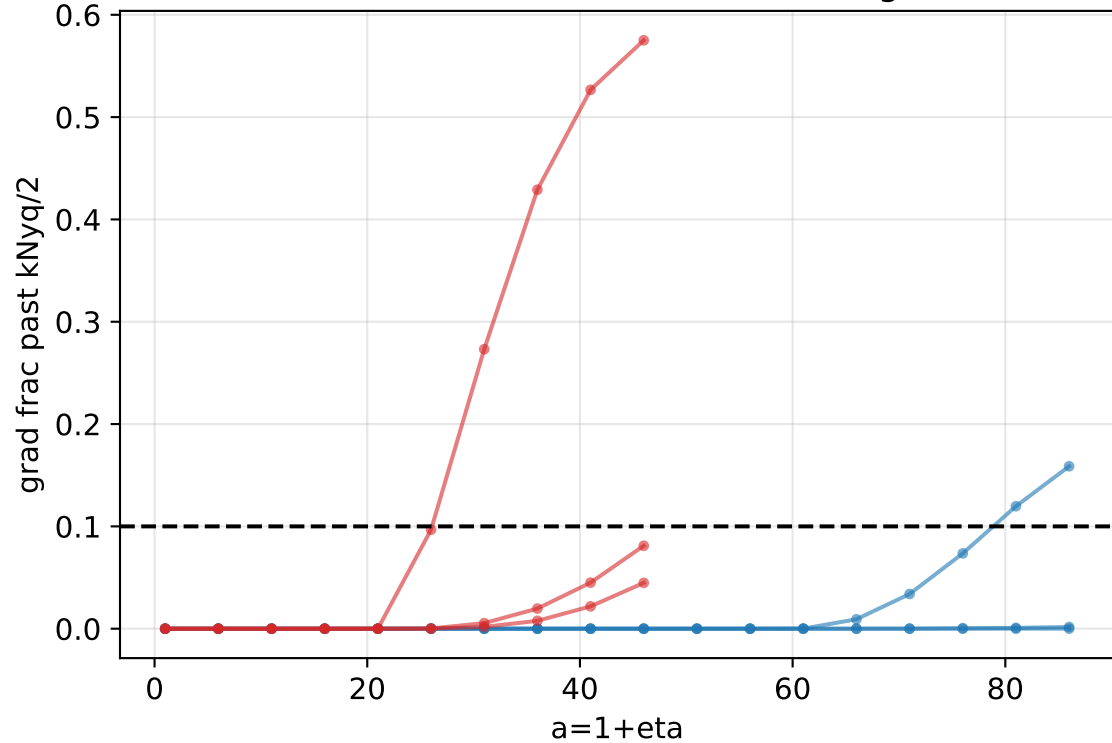
F \sim 0 until late roundoff aliasing
