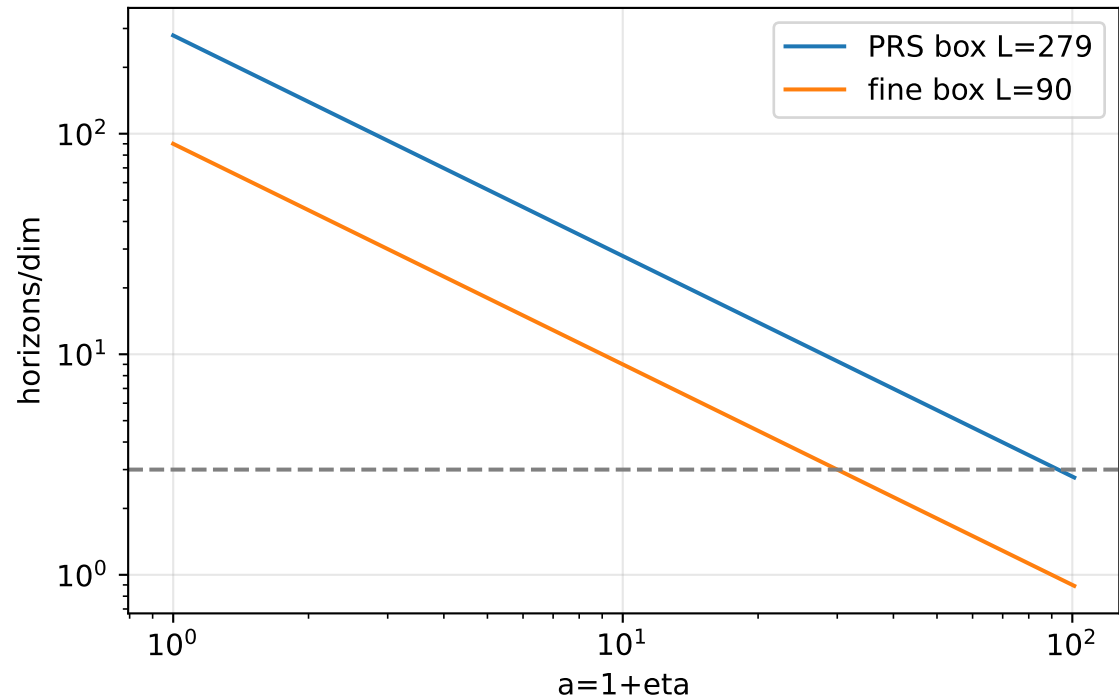
horizons \sim l_{\text{Side}}/a
