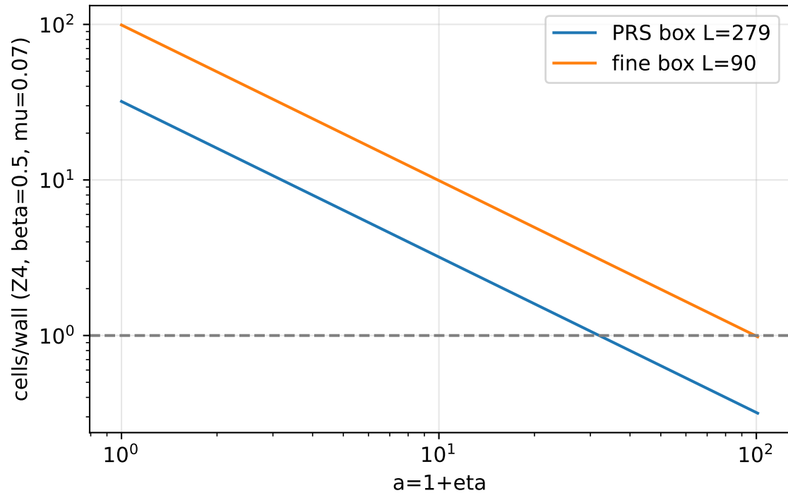
comoving cells/wall \sim 1/(\mu*a) (physical run)
