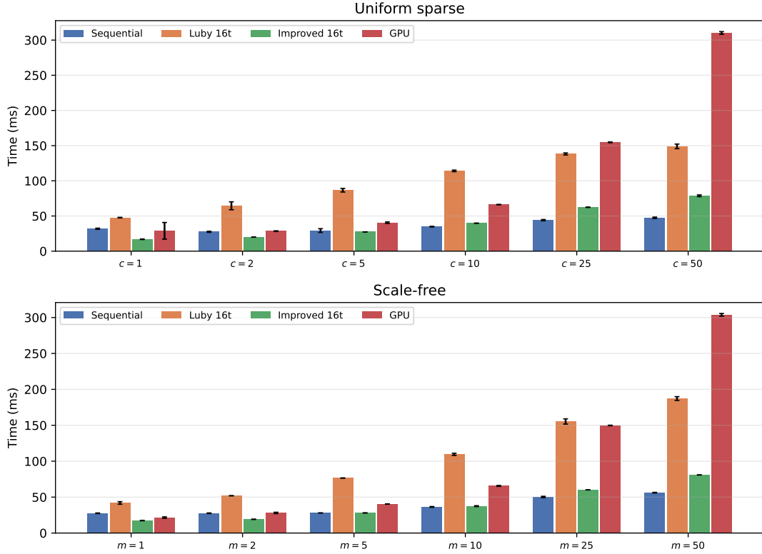
§3: Graph topology ( N = 5 \times 10^6 , 16 threads)
