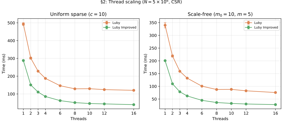
Figure 3: Performance scaling with the number of OpenMP threads ( N = 5 \cdot 10^6 ).
