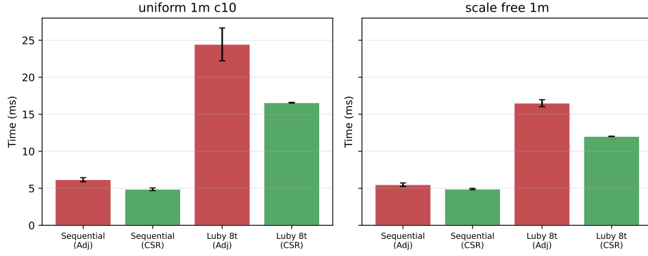
Figure 1: Performance comparison between CSR and standard adjacency list representation.
