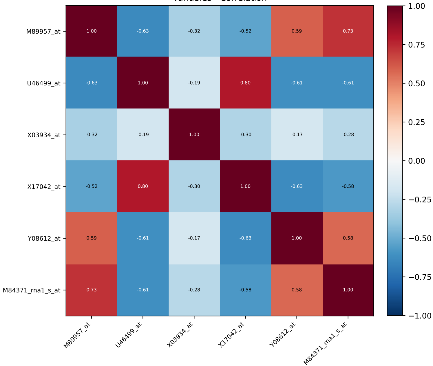
Variables - Correlation
