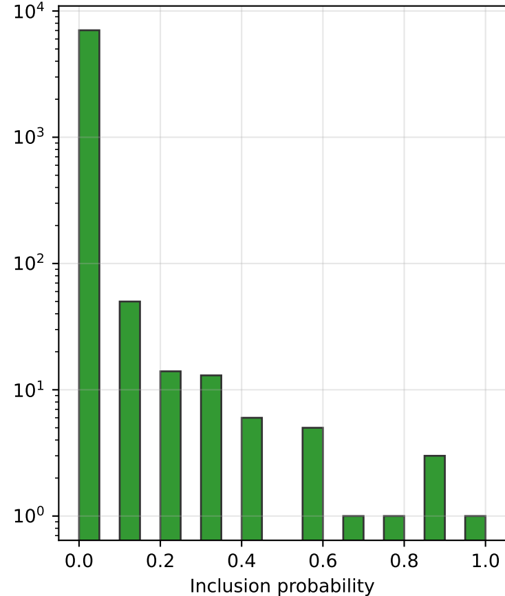
Lasso: inclusion probability distribution
