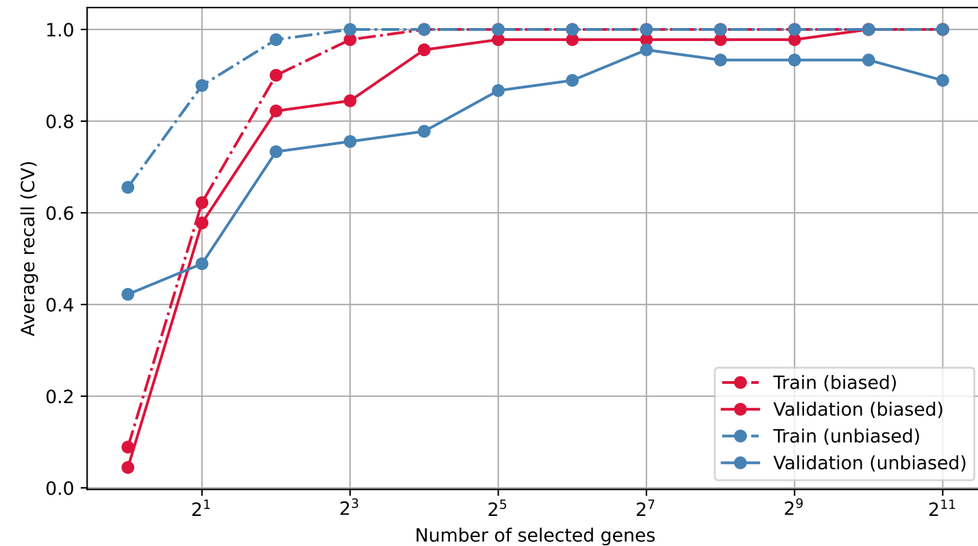
RFE
