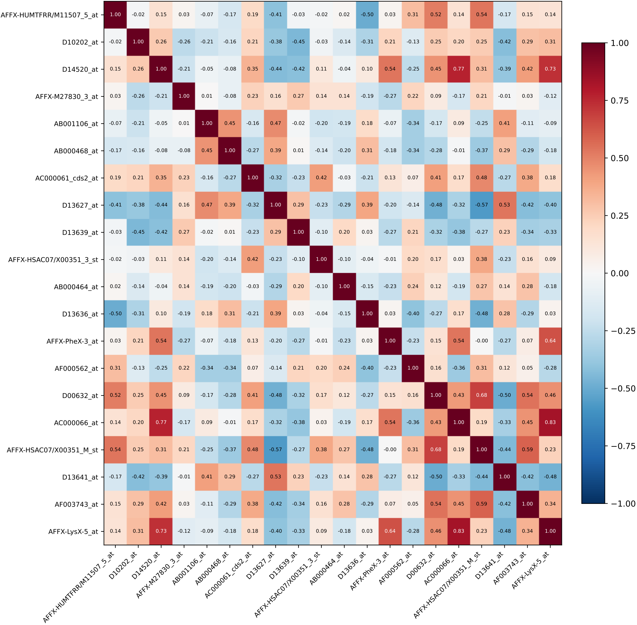
Variables - Correlation
