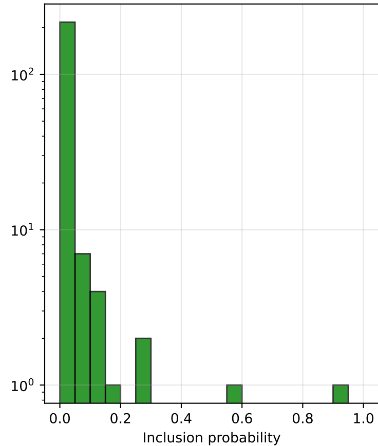
Lasso: inclusion probability distribution
