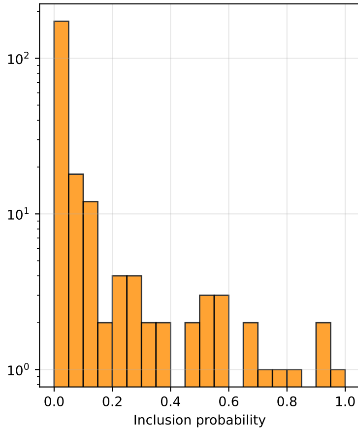
FDR (BH): inclusion probability distribution
