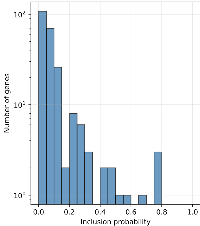
SVM-RFE: inclusion probability distribution
