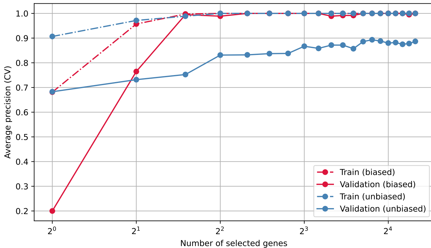
RFE
