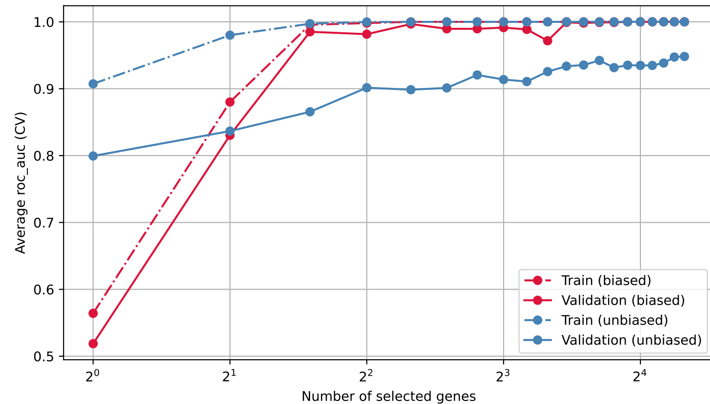
RFE
