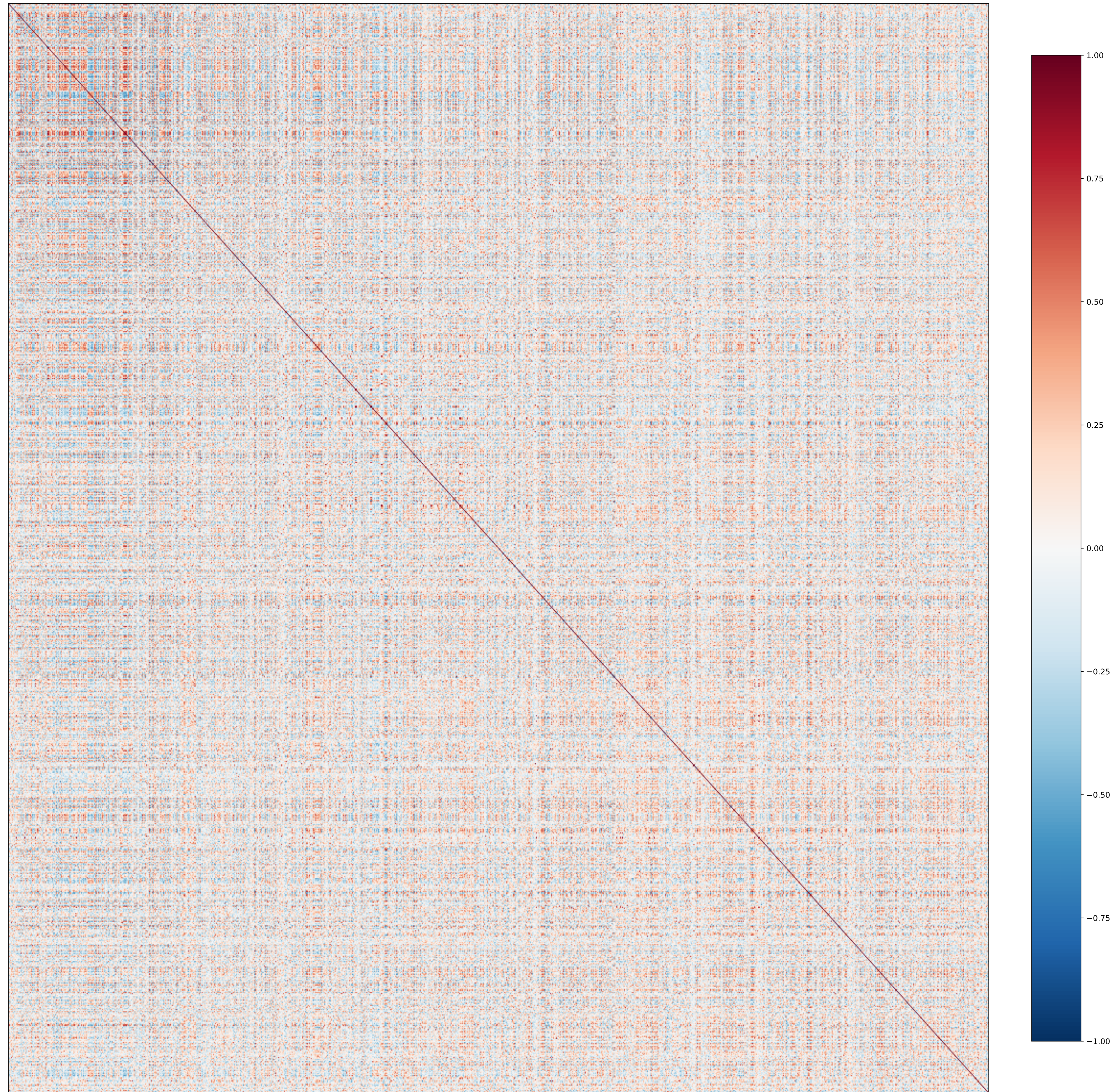
Variables - Correlation
